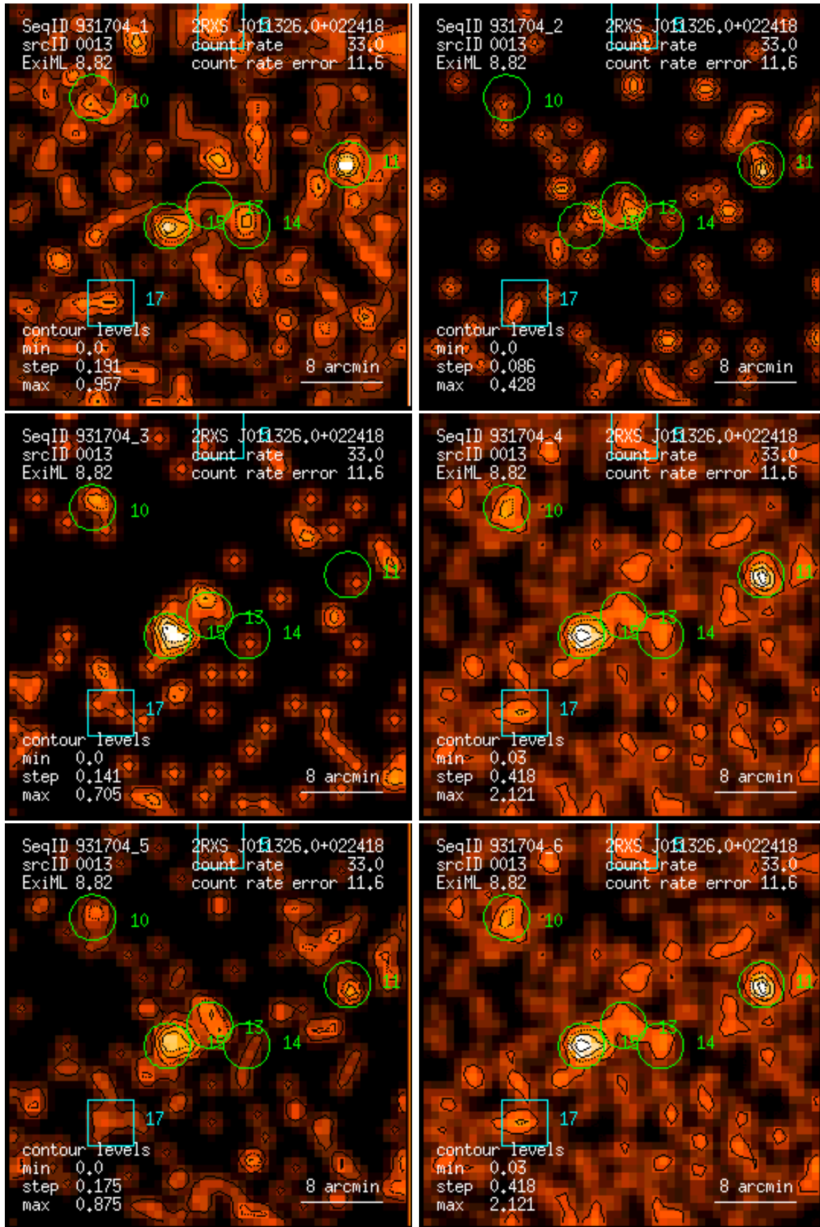
Figure 13: RASS 931704: detection 0013: band rate images, Gaussian filter: (1) PSPC channels 11 – 41, (2) 52 – 90, (3) 91 – 201, (4) 11 – 235, (5) 52 – 201, (6) 11 – 201. Broad band rates in counts/ks. Band rate contour levels in counts/ks/arcmin 2 .
