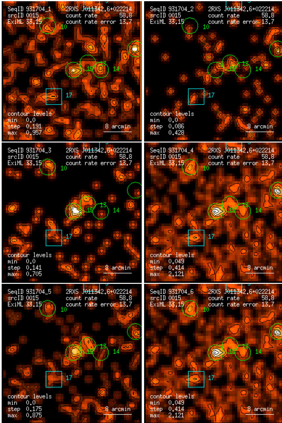
Figure 15: RASS 931704: detection 0015: band rate images, Gaussian filter: (1) PSPC channels 11 – 41, (2) 52 – 90, (3) 91 – 201, (4) 11 – 235, (5) 52 – 201, (6) 11 – 201. Broad band rates in counts/ks. Band rate contour levels in counts/ks/arcmin 2 .
