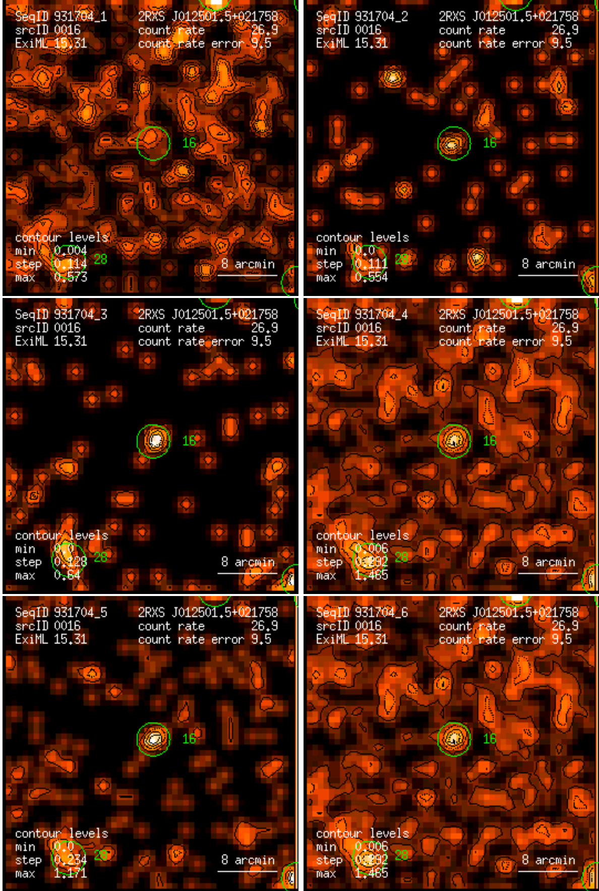
Figure 16: RASS 931704: detection 0016: band rate images, Gaussian filter: (1) PSPC channels 11 – 41, (2) 52 – 90, (3) 91 – 201, (4) 11 – 235, (5) 52 – 201, (6) 11 – 201. Broad band rates in counts/ks. Band rate contour levels in counts/ks/arcmin 2 .
