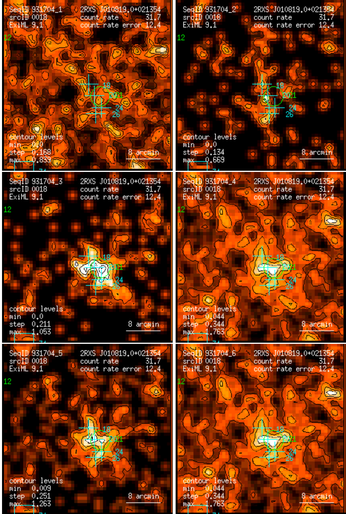
Figure 18: RASS 931704: detection 0018: band rate images, Gaussian filter: (1) PSPC channels 11 – 41, (2) 52 – 90, (3) 91 – 201, (4) 11 – 235, (5) 52 – 201, (6) 11 – 201. Broad band rates in counts/ks. Band rate contour levels in counts/ks/arcmin 2 .
