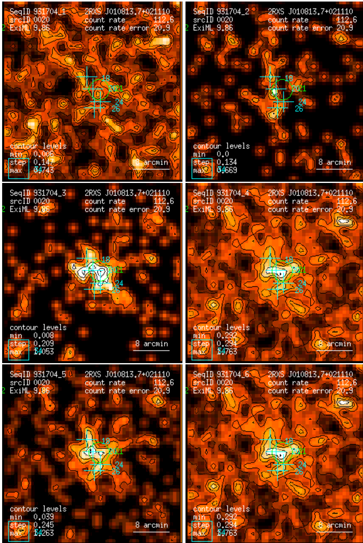
Figure 20: RASS 931704: detection 0020: band rate images, Gaussian filter: (1) PSPC channels 11 – 41, (2) 52 – 90, (3) 91 – 201, (4) 11 – 235, (5) 52 – 201, (6) 11 – 201. Broad band rates in counts/ks. Band rate contour levels in counts/ks/arcmin 2 .
