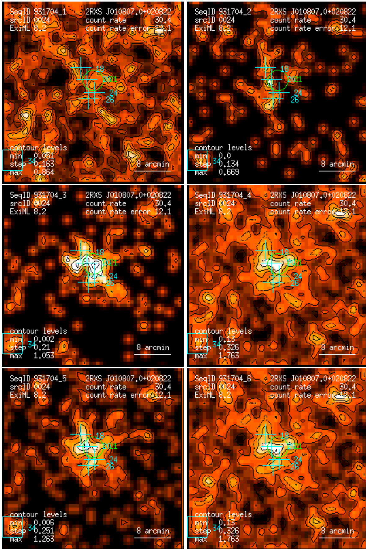
Figure 24: RASS 931704: detection 0024: band rate images, Gaussian filter: (1) PSPC channels 11 – 41, (2) 52 – 90, (3) 91 – 201, (4) 11 – 235, (5) 52 – 201, (6) 11 – 201. Broad band rates in counts/ks. Band rate contour levels in counts/ks/arcmin 2 .
