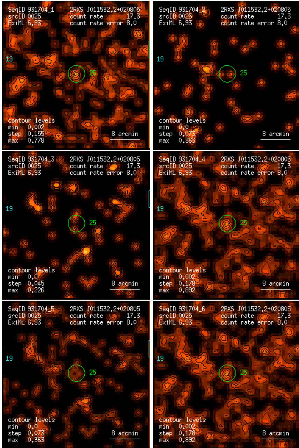
Figure 25: RASS 931704: detection 0025: band rate images, Gaussian filter: (1) PSPC channels 11 – 41, (2) 52 – 90, (3) 91 – 201, (4) 11 – 235, (5) 52 – 201, (6) 11 – 201. Broad band rates in counts/ks. Band rate contour levels in counts/ks/arcmin 2 .
