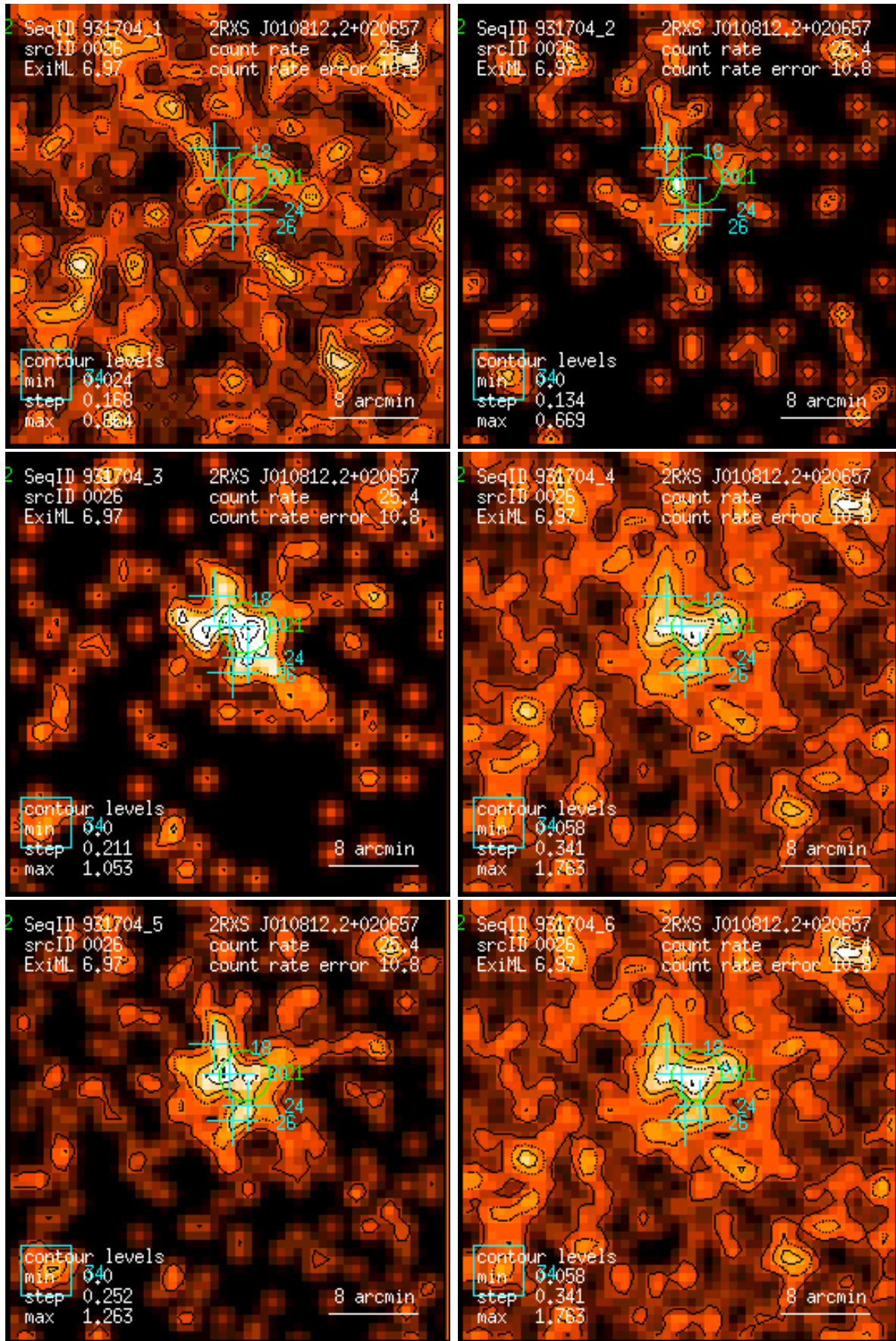
Figure 26: RASS 931704: detection 0026: band rate images, Gaussian filter: (1) PSPC channels 11 – 41, (2) 52 – 90, (3) 91 – 201, (4) 11 – 235, (5) 52 – 201, (6) 11 – 201. Broad band rates in counts/ks. Band rate contour levels in counts/ks/arcmin 2 .
