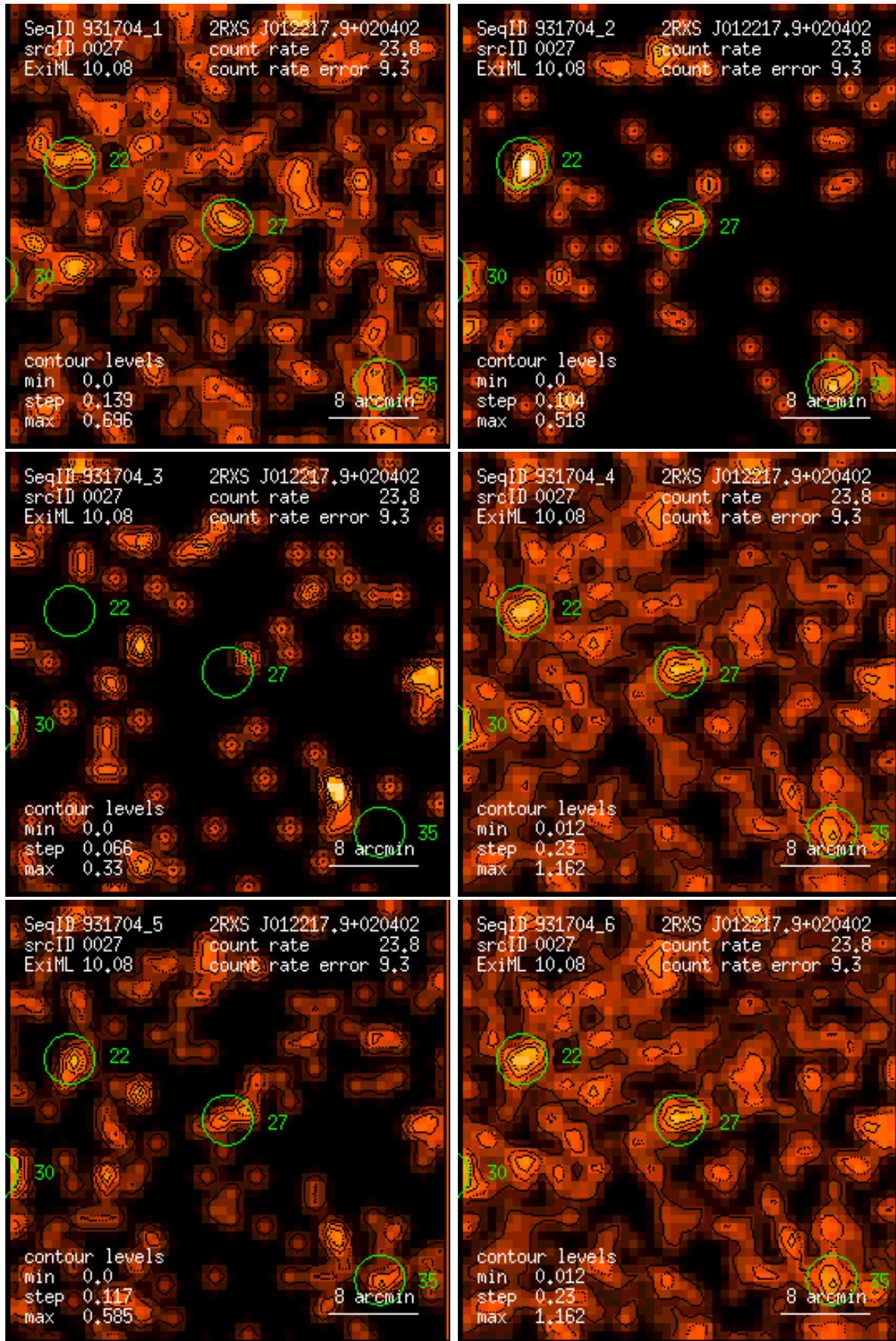
Figure 27: RASS 931704: detection 0027: band rate images, Gaussian filter: (1) PSPC channels 11 – 41, (2) 52 – 90, (3) 91 – 201, (4) 11 – 235, (5) 52 – 201, (6) 11 – 201. Broad band rates in counts/ks. Band rate contour levels in counts/ks/arcmin 2 .
