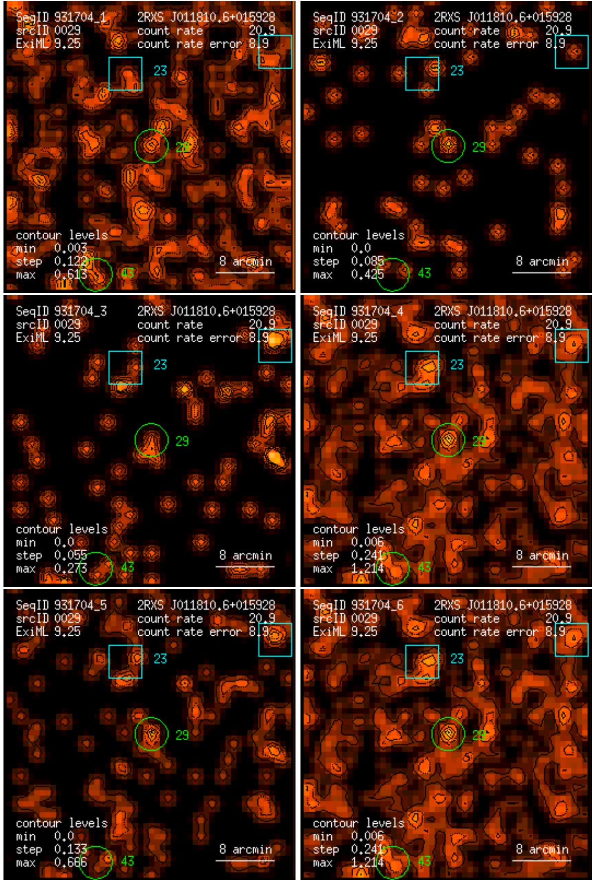
Figure 29: RASS 931704: detection 0029: band rate images, Gaussian filter: (1) PSPC channels 11 – 41, (2) 52 – 90, (3) 91 – 201, (4) 11 – 235, (5) 52 – 201, (6) 11 – 201. Broad band rates in counts/ks. Band rate contour levels in counts/ks/arcmin 2 .
