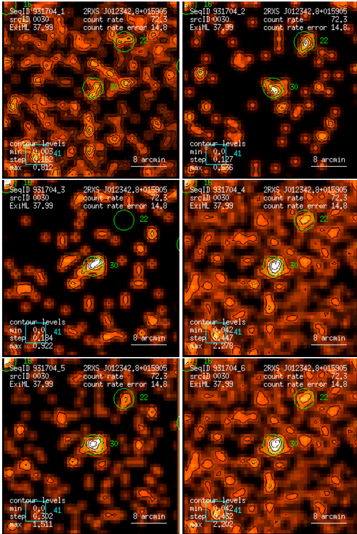
Figure 30: RASS 931704: detection 0030: band rate images, Gaussian filter: (1) PSPC channels 11 – 41, (2) 52 – 90, (3) 91 – 201, (4) 11 – 235, (5) 52 – 201, (6) 11 – 201. Broad band rates in counts/ks. Band rate contour levels in counts/ks/arcmin 2 .
