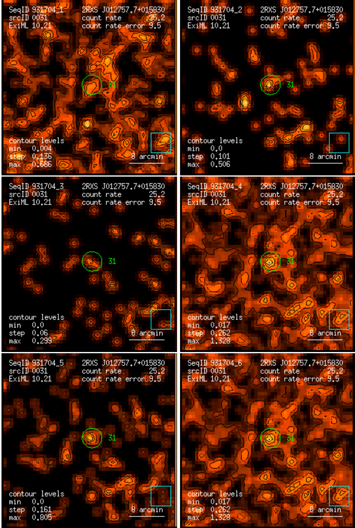
Figure 31: RASS 931704: detection 0031: band rate images, Gaussian filter: (1) PSPC channels 11 – 41, (2) 52 – 90, (3) 91 – 201, (4) 11 – 235, (5) 52 – 201, (6) 11 – 201. Broad band rates in counts/ks. Band rate contour levels in counts/ks/arcmin 2 .
