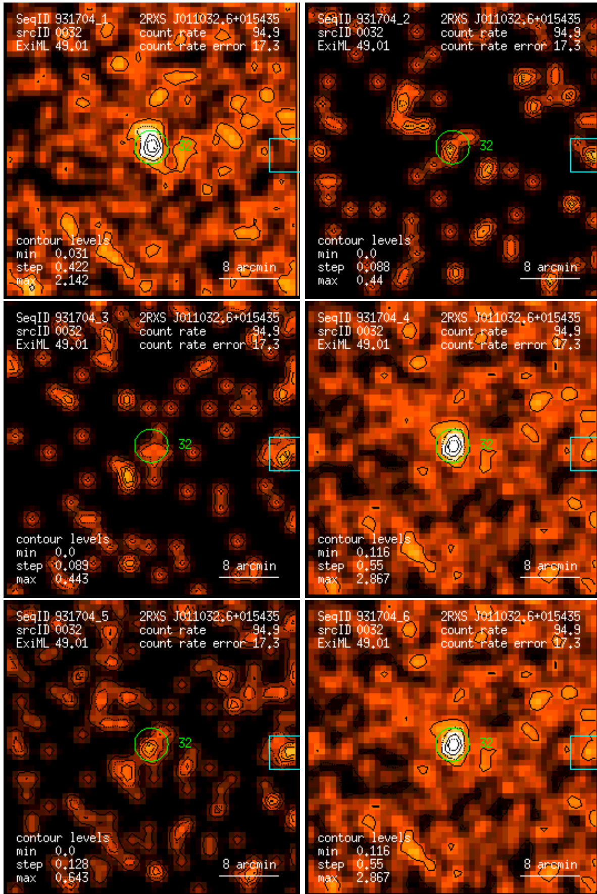
Figure 32: RASS 931704: detection 0032: band rate images, Gaussian filter: (1) PSPC channels 11 – 41, (2) 52 – 90, (3) 91 – 201, (4) 11 – 235, (5) 52 – 201, (6) 11 – 201. Broad band rates in counts/ks. Band rate contour levels in counts/ks/arcmin 2 .
