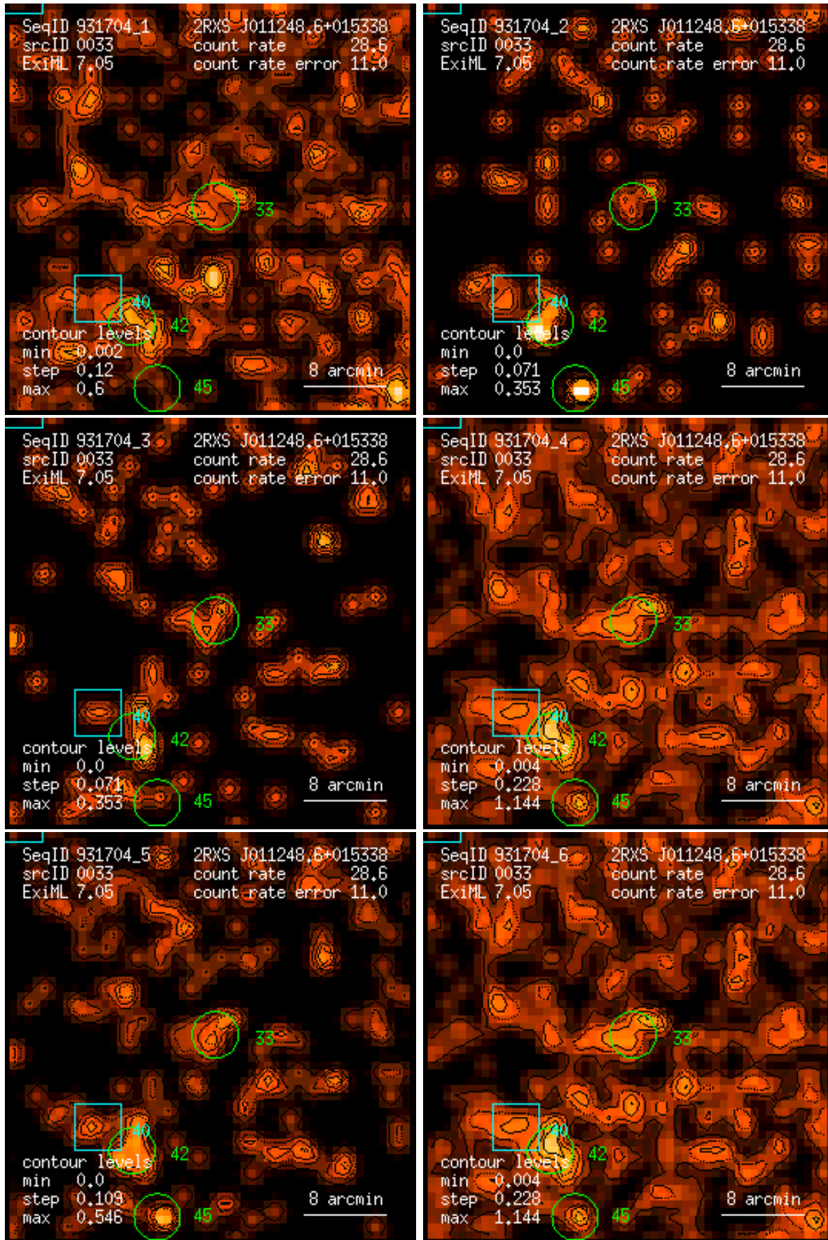
Figure 33: RASS 931704: detection 0033: band rate images, Gaussian filter: (1) PSPC channels 11 – 41, (2) 52 – 90, (3) 91 – 201, (4) 11 – 235, (5) 52 – 201, (6) 11 – 201. Broad band rates in counts/ks. Band rate contour levels in counts/ks/arcmin 2 .
