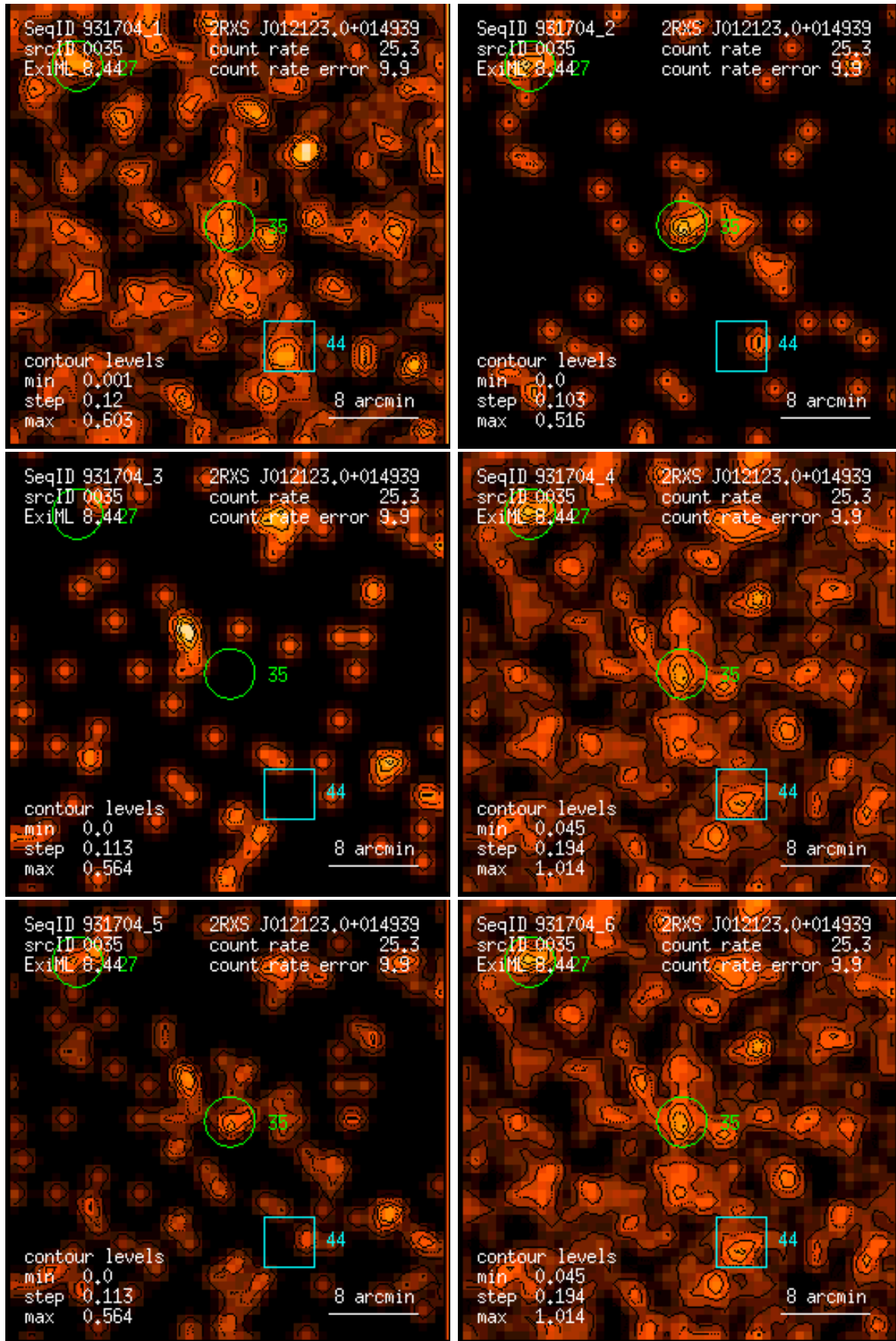
Figure 35: RASS 931704: detection 0035: band rate images, Gaussian filter: (1) PSPC channels 11 – 41, (2) 52 – 90, (3) 91 – 201, (4) 11 – 235, (5) 52 – 201, (6) 11 – 201. Broad band rates in counts/ks. Band rate contour levels in counts/ks/arcmin 2 .
