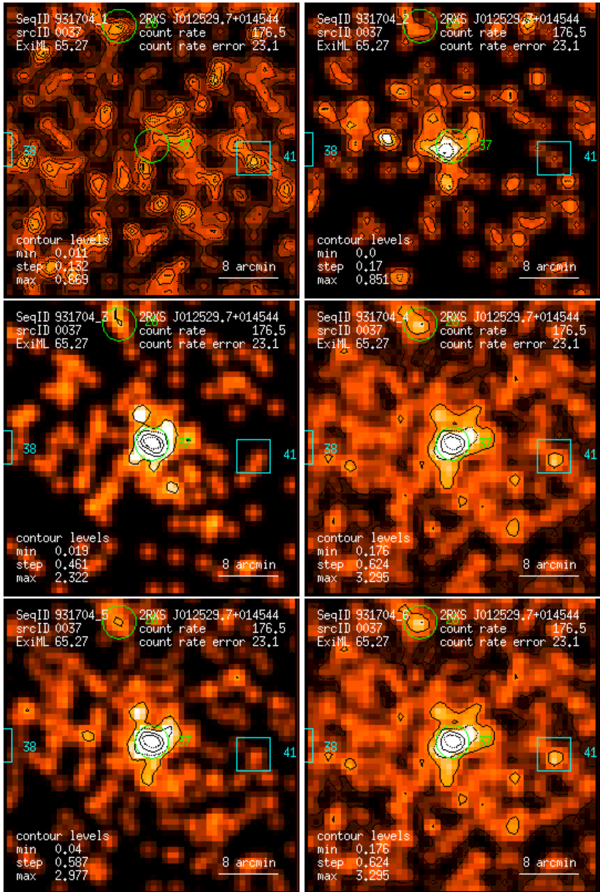
Figure 37: RASS 931704: detection 0037: band rate images, Gaussian filter: (1) PSPC channels 11 – 41, (2) 52 – 90, (3) 91 – 201, (4) 11 – 235, (5) 52 – 201, (6) 11 – 201. Broad band rates in counts/ks. Band rate contour levels in counts/ks/arcmin 2 .
