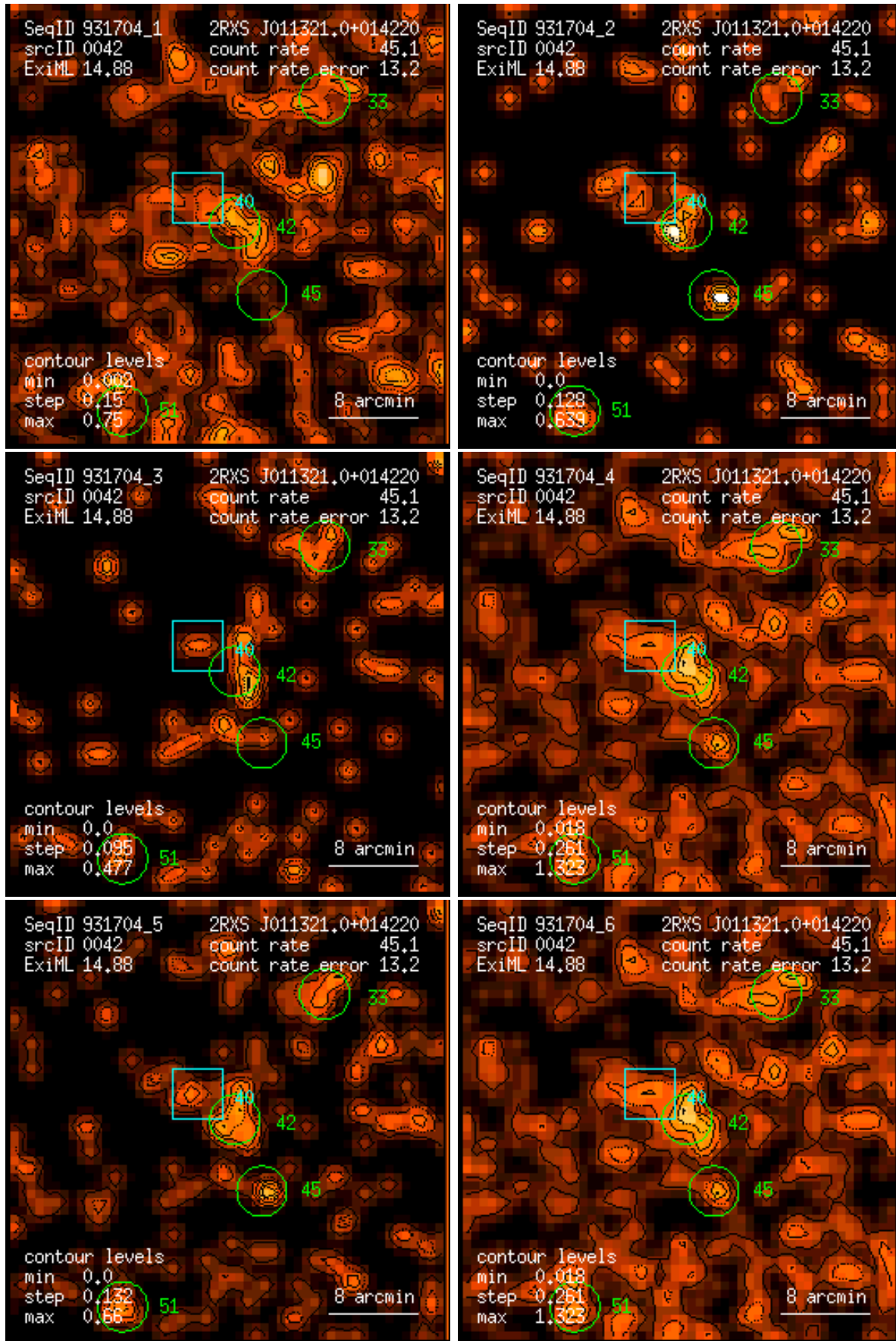
Figure 42: RASS 931704: detection 0042: band rate images, Gaussian filter: (1) PSPC channels 11 – 41, (2) 52 – 90, (3) 91 – 201, (4) 11 – 235, (5) 52 – 201, (6) 11 – 201. Broad band rates in counts/ks. Band rate contour levels in counts/ks/arcmin 2 .
