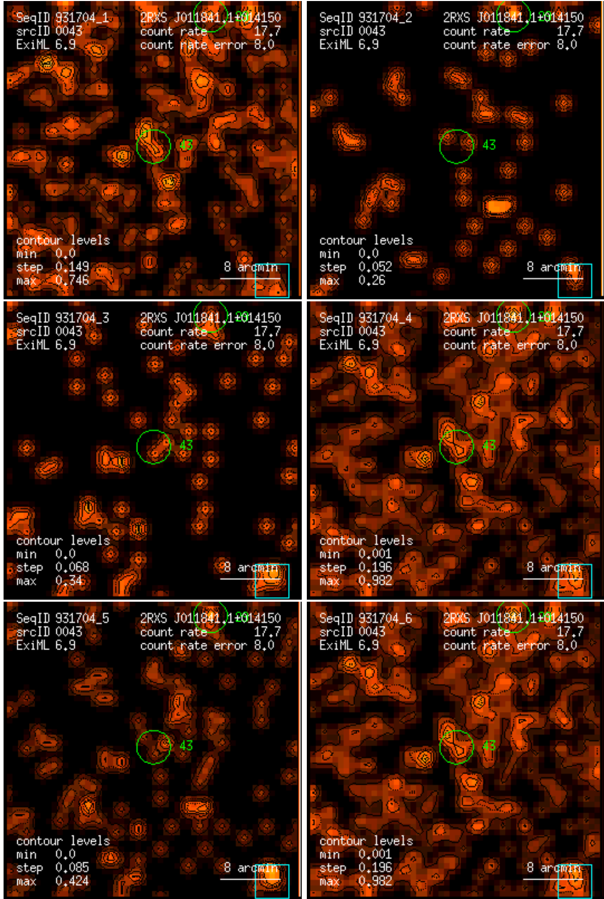
Figure 43: RASS 931704: detection 0043: band rate images, Gaussian filter: (1) PSPC channels 11 – 41, (2) 52 – 90, (3) 91 – 201, (4) 11 – 235, (5) 52 – 201, (6) 11 – 201. Broad band rates in counts/ks. Band rate contour levels in counts/ks/arcmin 2 .
