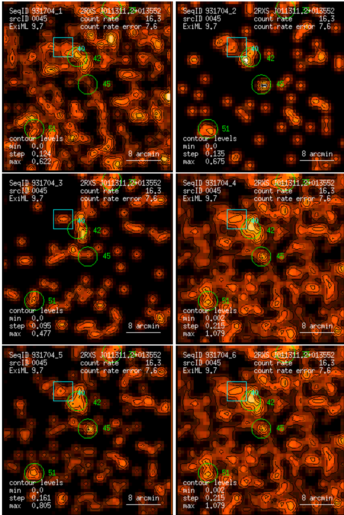
Figure 45: RASS 931704: detection 0045: band rate images, Gaussian filter: (1) PSPC channels 11 – 41, (2) 52 – 90, (3) 91 – 201, (4) 11 – 235, (5) 52 – 201, (6) 11 – 201. Broad band rates in counts/ks. Band rate contour levels in counts/ks/arcmin 2 .
