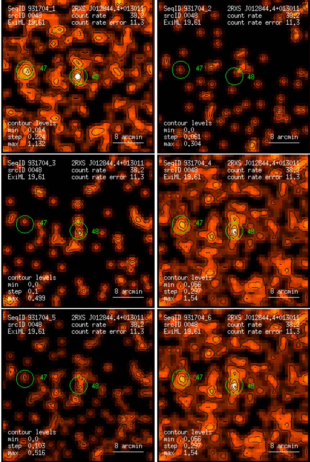
Figure 48: RASS 931704: detection 0048: band rate images, Gaussian filter: (1) PSPC channels 11 – 41, (2) 52 – 90, (3) 91 – 201, (4) 11 – 235, (5) 52 – 201, (6) 11 – 201. Broad band rates in counts/ks. Band rate contour levels in counts/ks/arcmin 2 .
