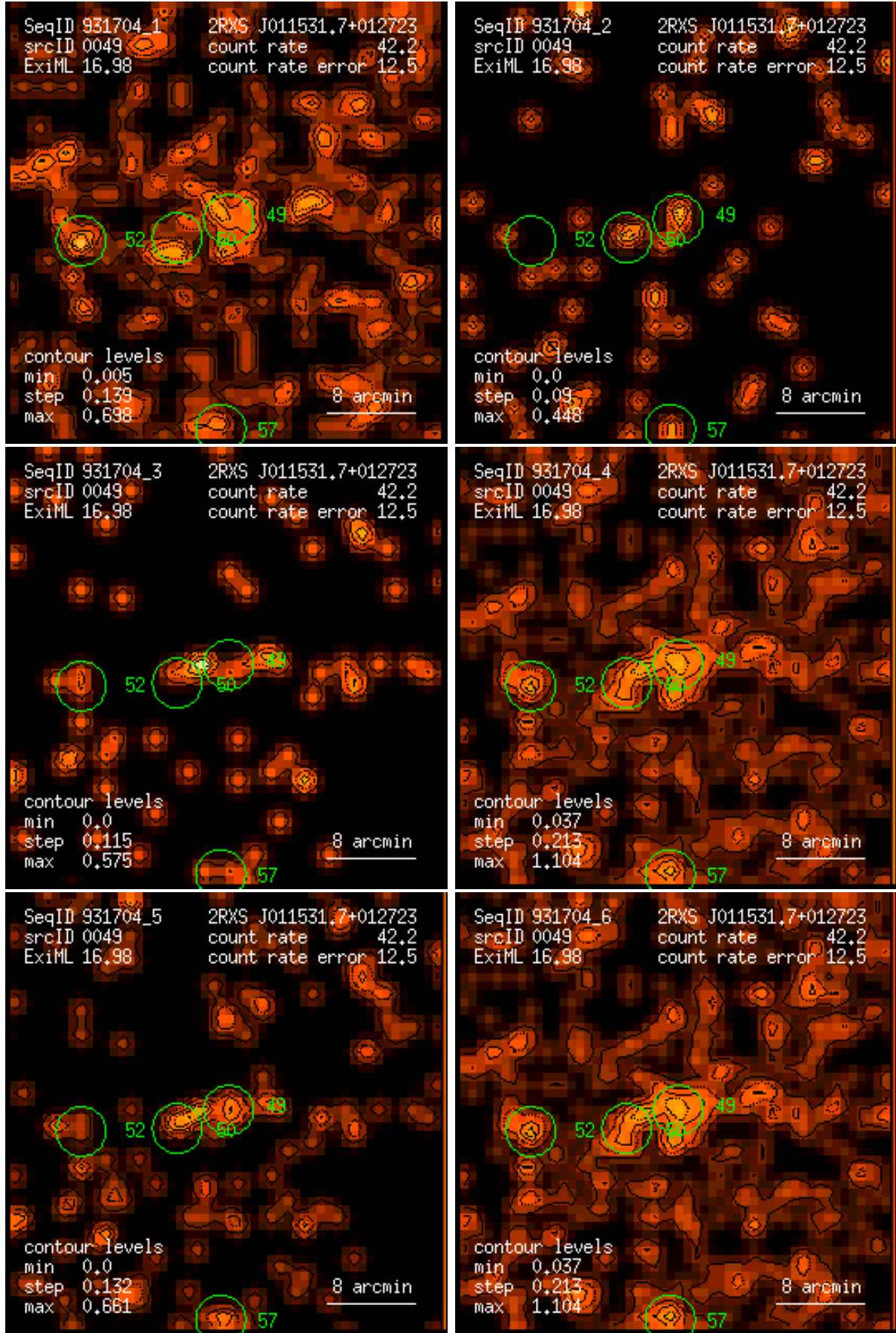
Figure 49: RASS 931704: detection 0049: band rate images, Gaussian filter: (1) PSPC channels 11 – 41, (2) 52 – 90, (3) 91 – 201, (4) 11 – 235, (5) 52 – 201, (6) 11 – 201. Broad band rates in counts/ks. Band rate contour levels in counts/ks/arcmin 2 .
