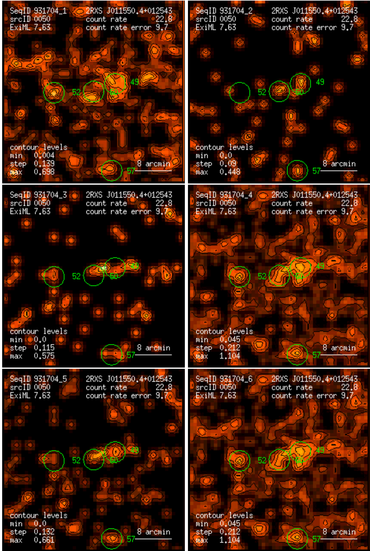
Figure 50: RASS 931704: detection 0050: band rate images, Gaussian filter: (1) PSPC channels 11 – 41, (2) 52 – 90, (3) 91 – 201, (4) 11 – 235, (5) 52 – 201, (6) 11 – 201. Broad band rates in counts/ks. Band rate contour levels in counts/ks/arcmin 2 .
