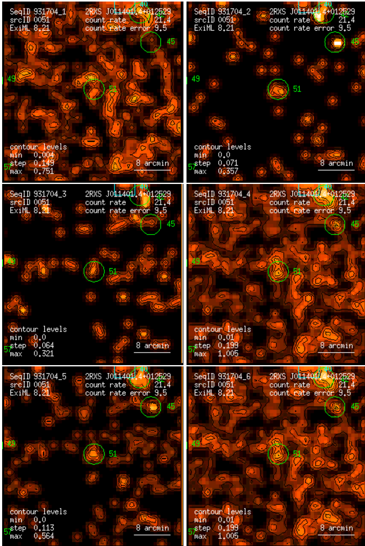
Figure 51: RASS 931704: detection 0051: band rate images, Gaussian filter: (1) PSPC channels 11 – 41, (2) 52 – 90, (3) 91 – 201, (4) 11 – 235, (5) 52 – 201, (6) 11 – 201. Broad band rates in counts/ks. Band rate contour levels in counts/ks/arcmin 2 .
