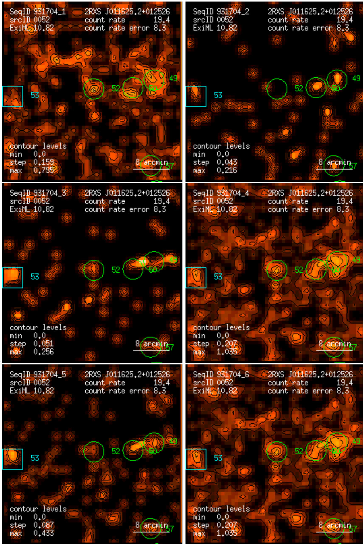
Figure 52: RASS 931704: detection 0052: band rate images, Gaussian filter: (1) PSPC channels 11 – 41, (2) 52 – 90, (3) 91 – 201, (4) 11 – 235, (5) 52 – 201, (6) 11 – 201. Broad band rates in counts/ks. Band rate contour levels in counts/ks/arcmin 2 .
