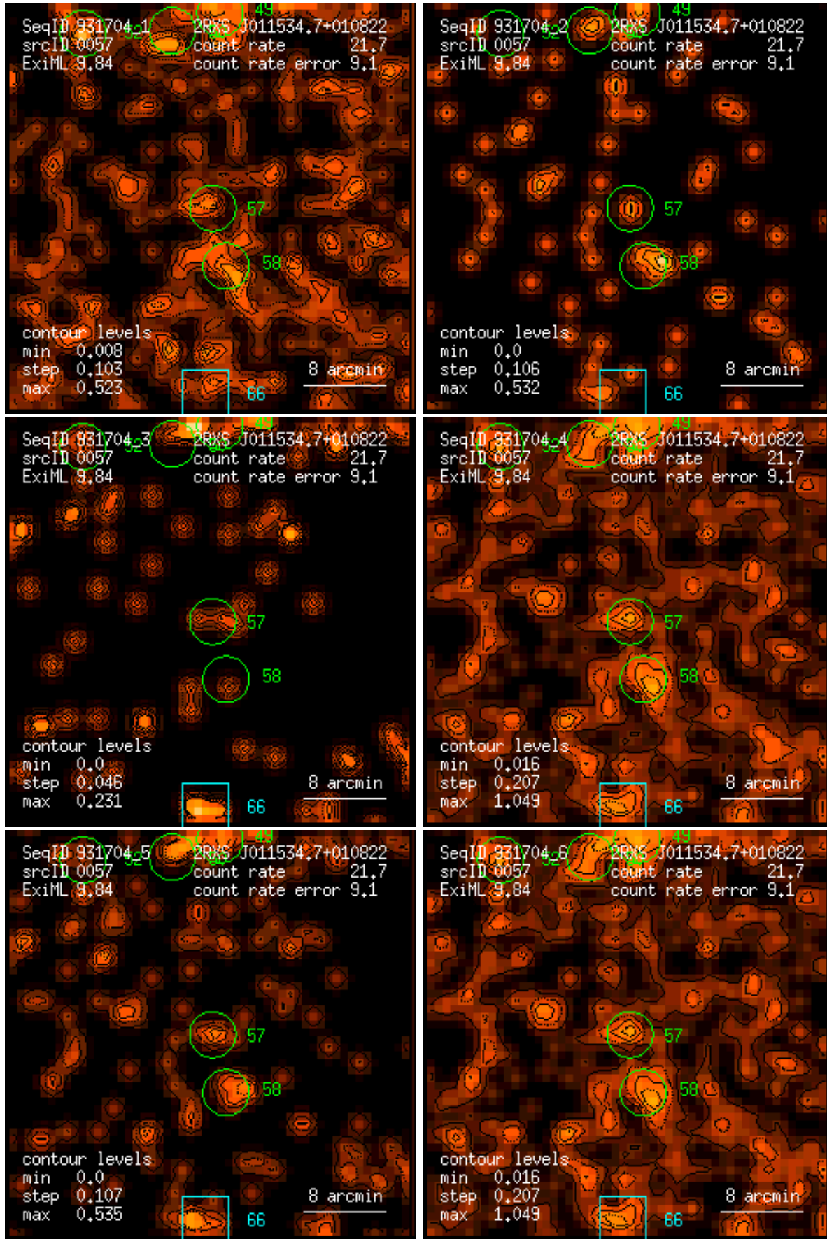
Figure 57: RASS 931704: detection 0057: band rate images, Gaussian filter: (1) PSPC channels 11 – 41, (2) 52 – 90, (3) 91 – 201, (4) 11 – 235, (5) 52 – 201, (6) 11 – 201. Broad band rates in counts/ks. Band rate contour levels in counts/ks/arcmin 2 .
