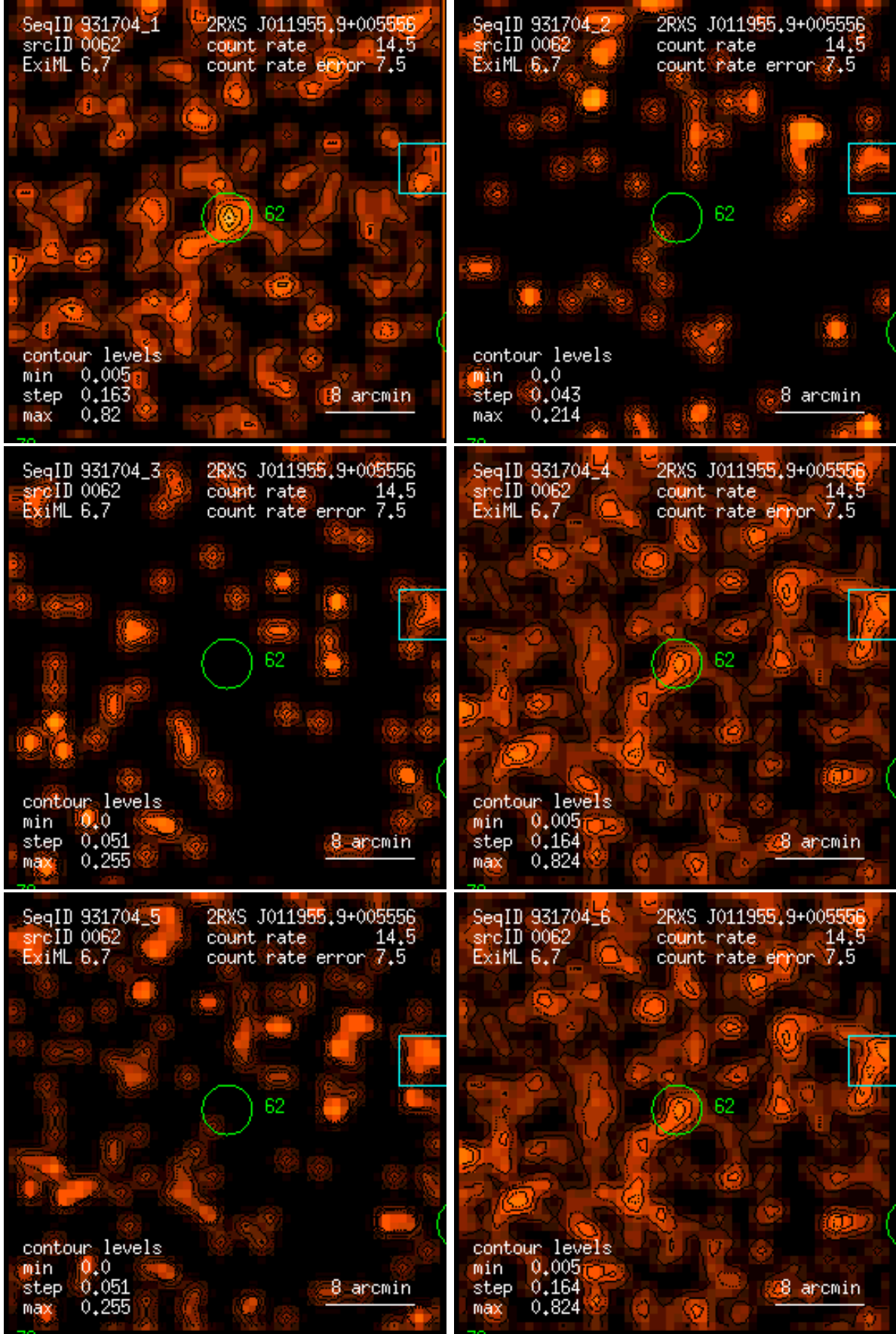
Figure 62: RASS 931704: detection 0062: band rate images, Gaussian filter: (1) PSPC channels 11 – 41, (2) 52 – 90, (3) 91 – 201, (4) 11 – 235, (5) 52 – 201, (6) 11 – 201. Broad band rates in counts/ks. Band rate contour levels in counts/ks/arcmin 2 .
