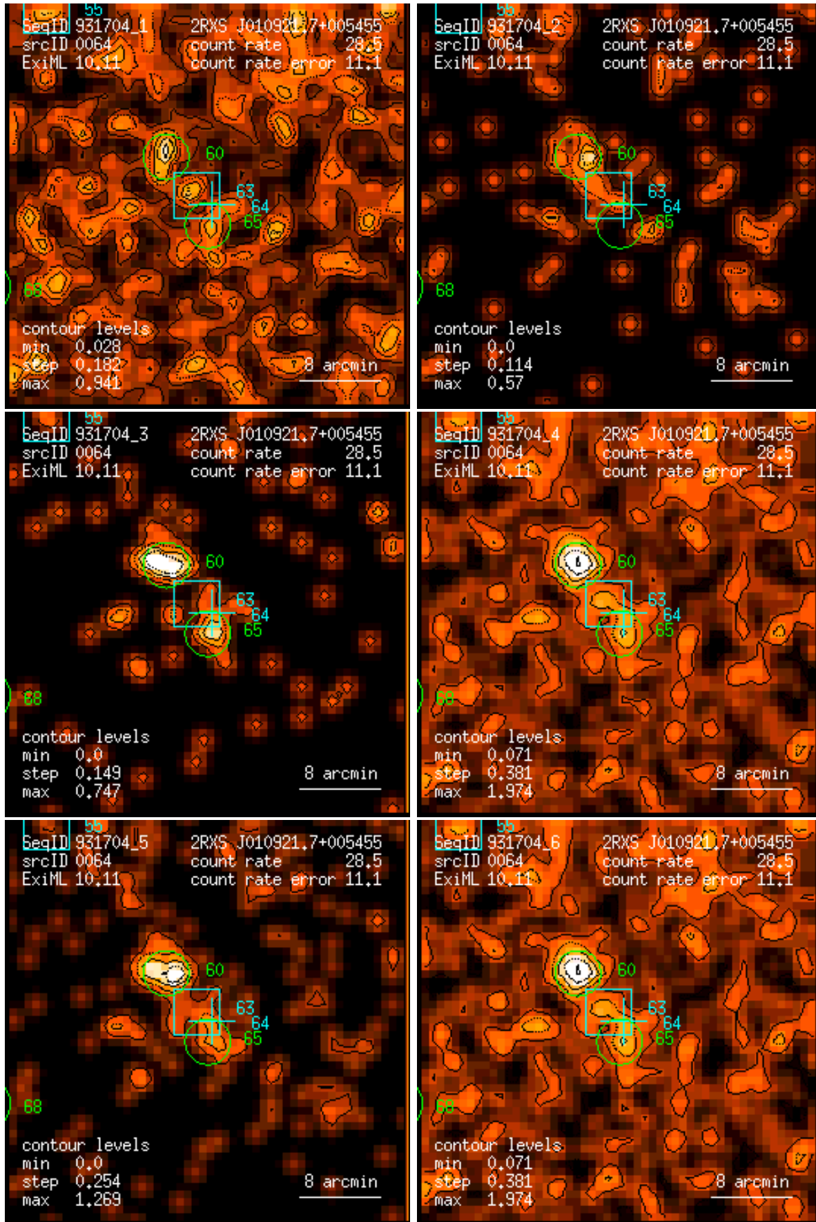
Figure 64: RASS 931704: detection 0064: band rate images, Gaussian filter: (1) PSPC channels 11 – 41, (2) 52 – 90, (3) 91 – 201, (4) 11 – 235, (5) 52 – 201, (6) 11 – 201. Broad band rates in counts/ks. Band rate contour levels in counts/ks/arcmin 2 .
