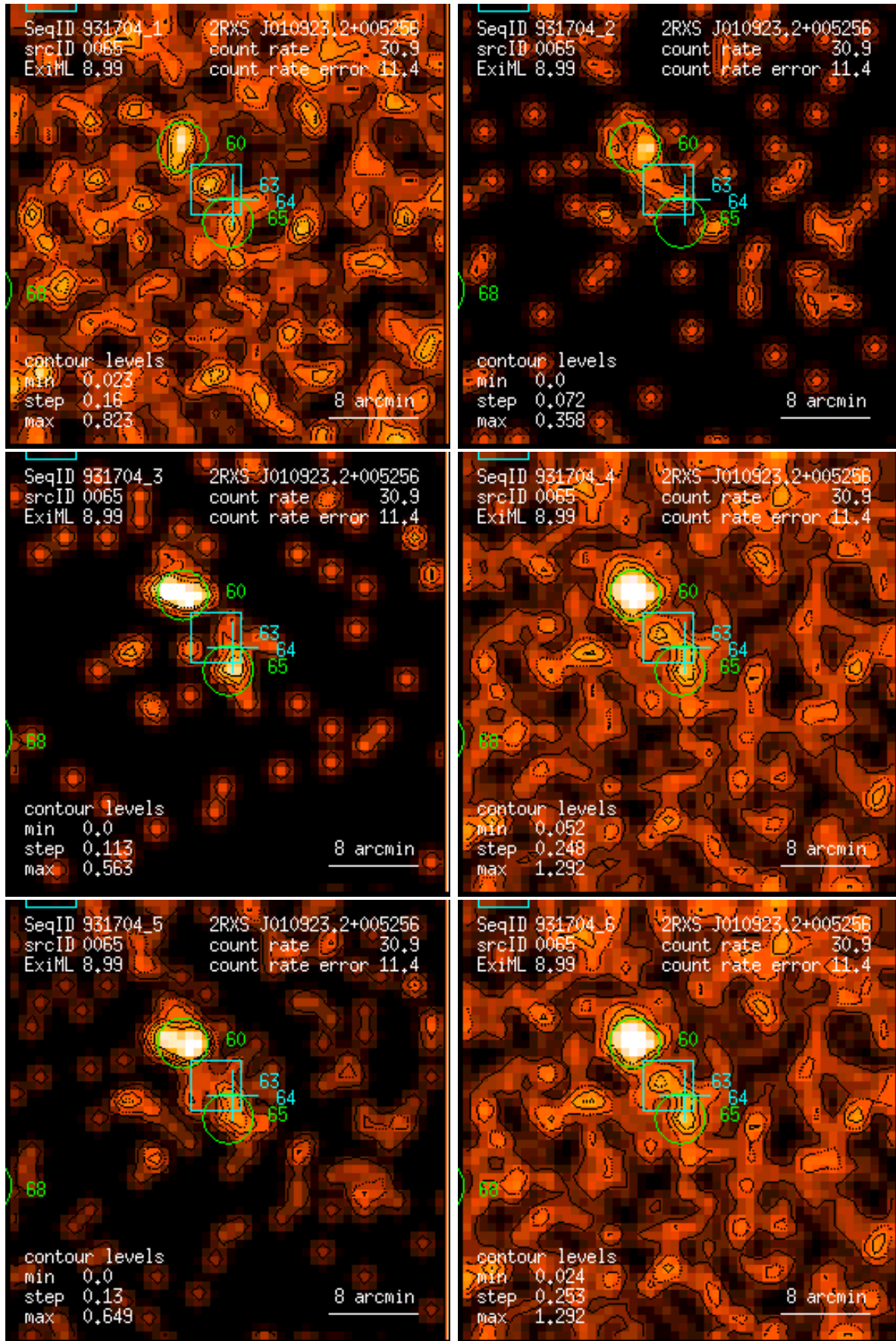
Figure 65: RASS 931704: detection 0065: band rate images, Gaussian filter: (1) PSPC channels 11 – 41, (2) 52 – 90, (3) 91 – 201, (4) 11 – 235, (5) 52 – 201, (6) 11 – 201. Broad band rates in counts/ks. Band rate contour levels in counts/ks/arcmin 2 .
