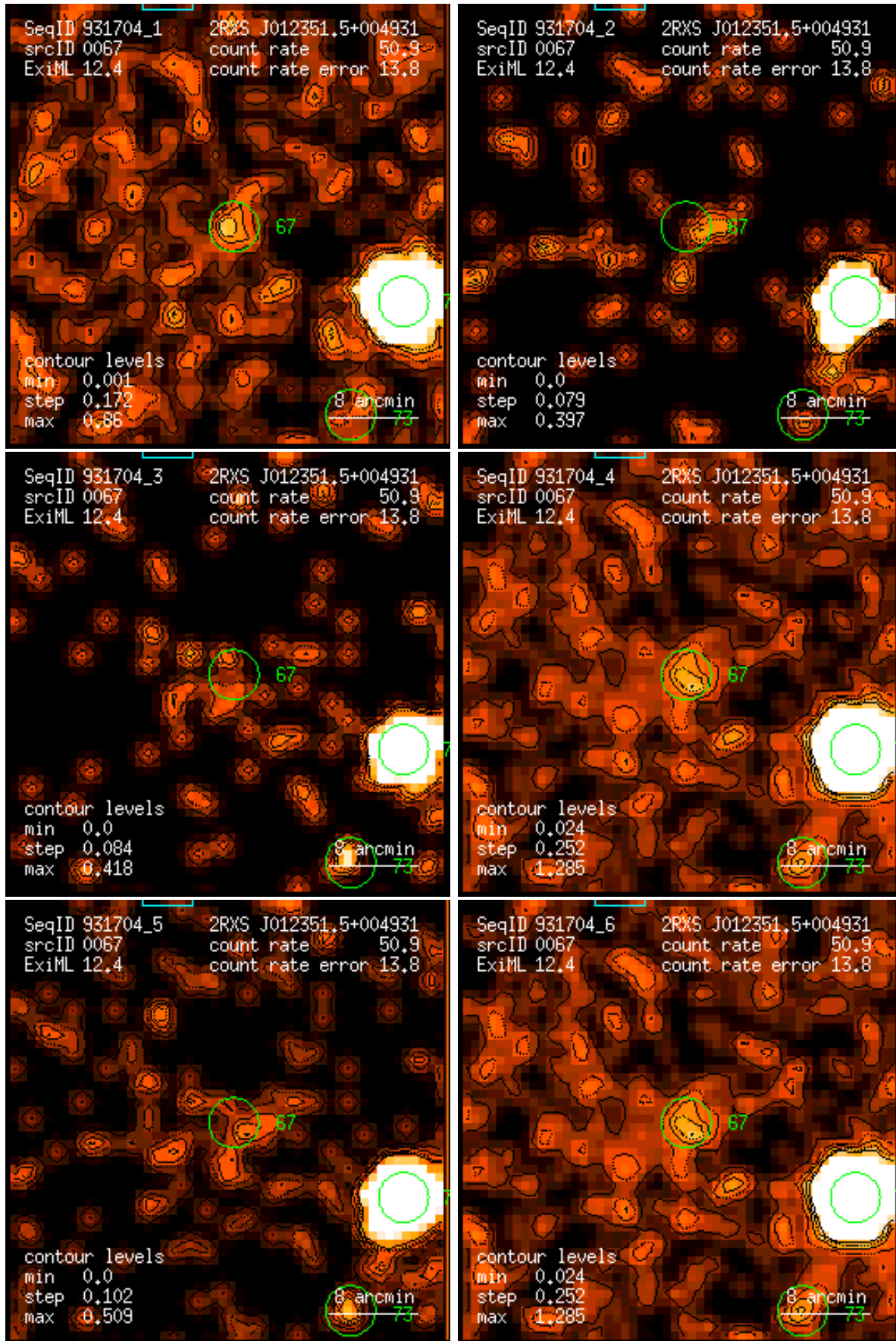
Figure 67: RASS 931704: detection 0067: band rate images, Gaussian filter: (1) PSPC channels 11 – 41, (2) 52 – 90, (3) 91 – 201, (4) 11 – 235, (5) 52 – 201, (6) 11 – 201. Broad band rates in counts/ks. Band rate contour levels in counts/ks/arcmin 2 .
