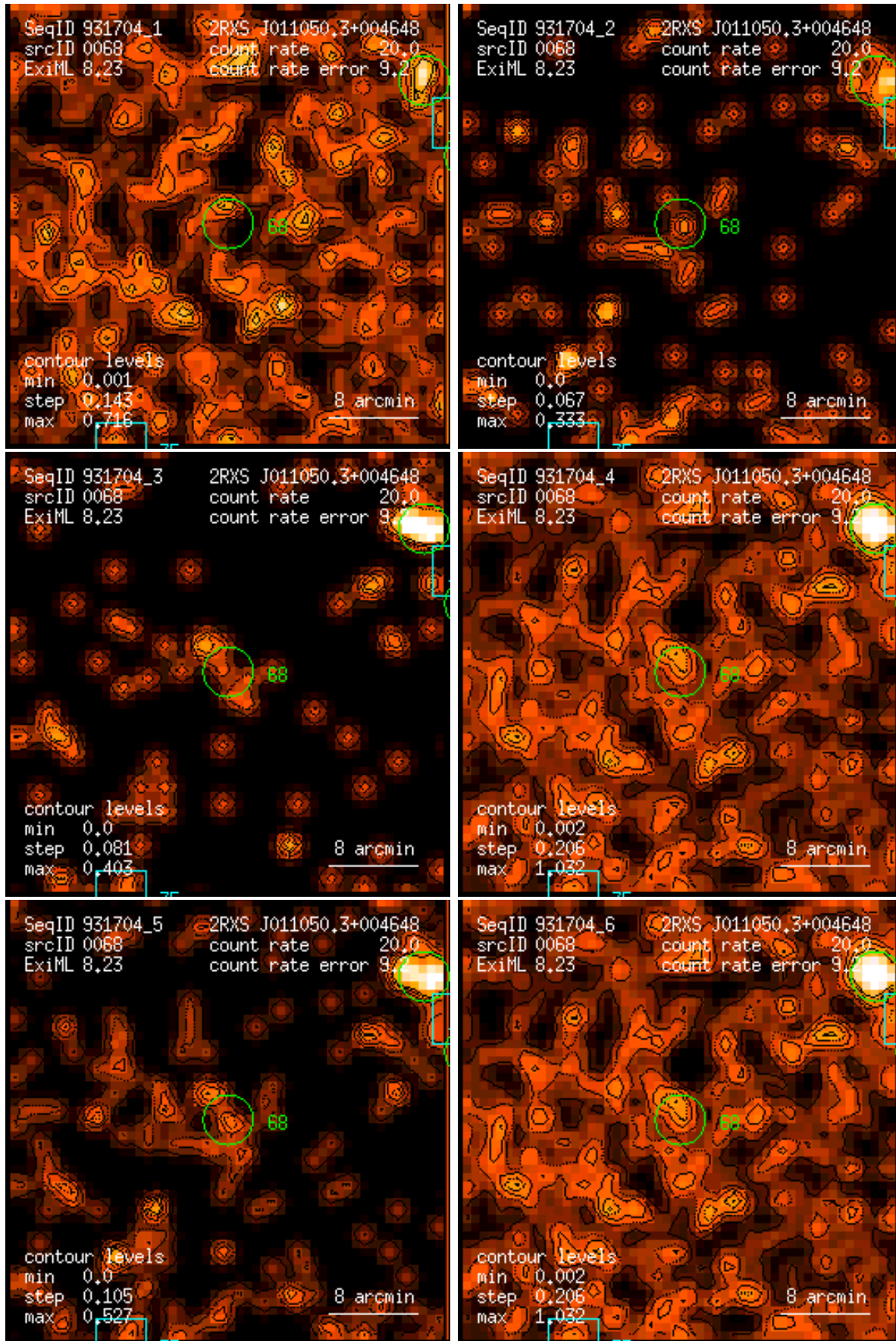
Figure 68: RASS 931704: detection 0068: band rate images, Gaussian filter: (1) PSPC channels 11 – 41, (2) 52 – 90, (3) 91 – 201, (4) 11 – 235, (5) 52 – 201, (6) 11 – 201. Broad band rates in counts/ks. Band rate contour levels in counts/ks/arcmin 2 .
