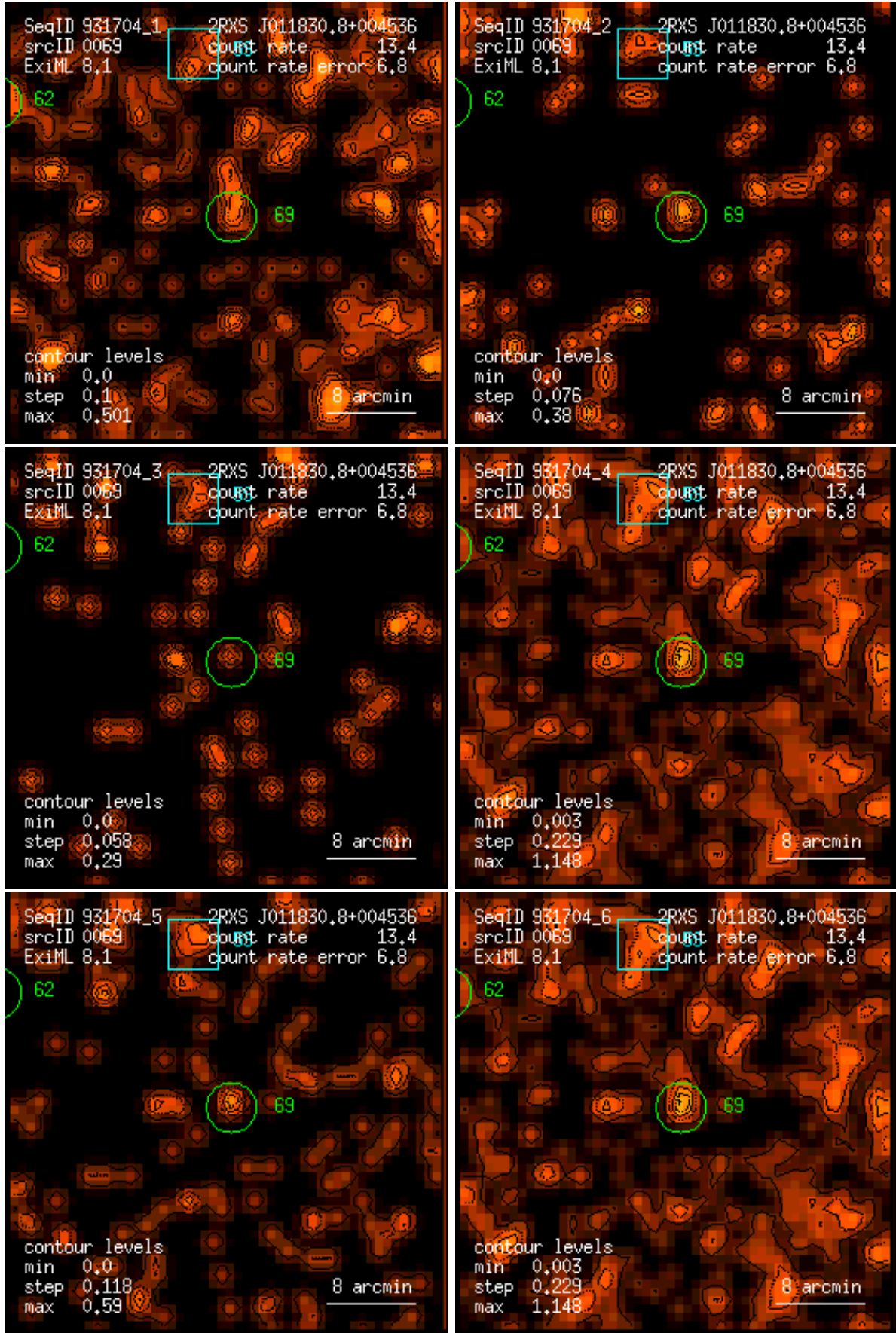
Figure 69: RASS 931704: detection 0069: band rate images, Gaussian filter: (1) PSPC channels 11 – 41, (2) 52 – 90, (3) 91 – 201, (4) 11 – 235, (5) 52 – 201, (6) 11 – 201. Broad band rates in counts/ks. Band rate contour levels in counts/ks/arcmin 2 .
