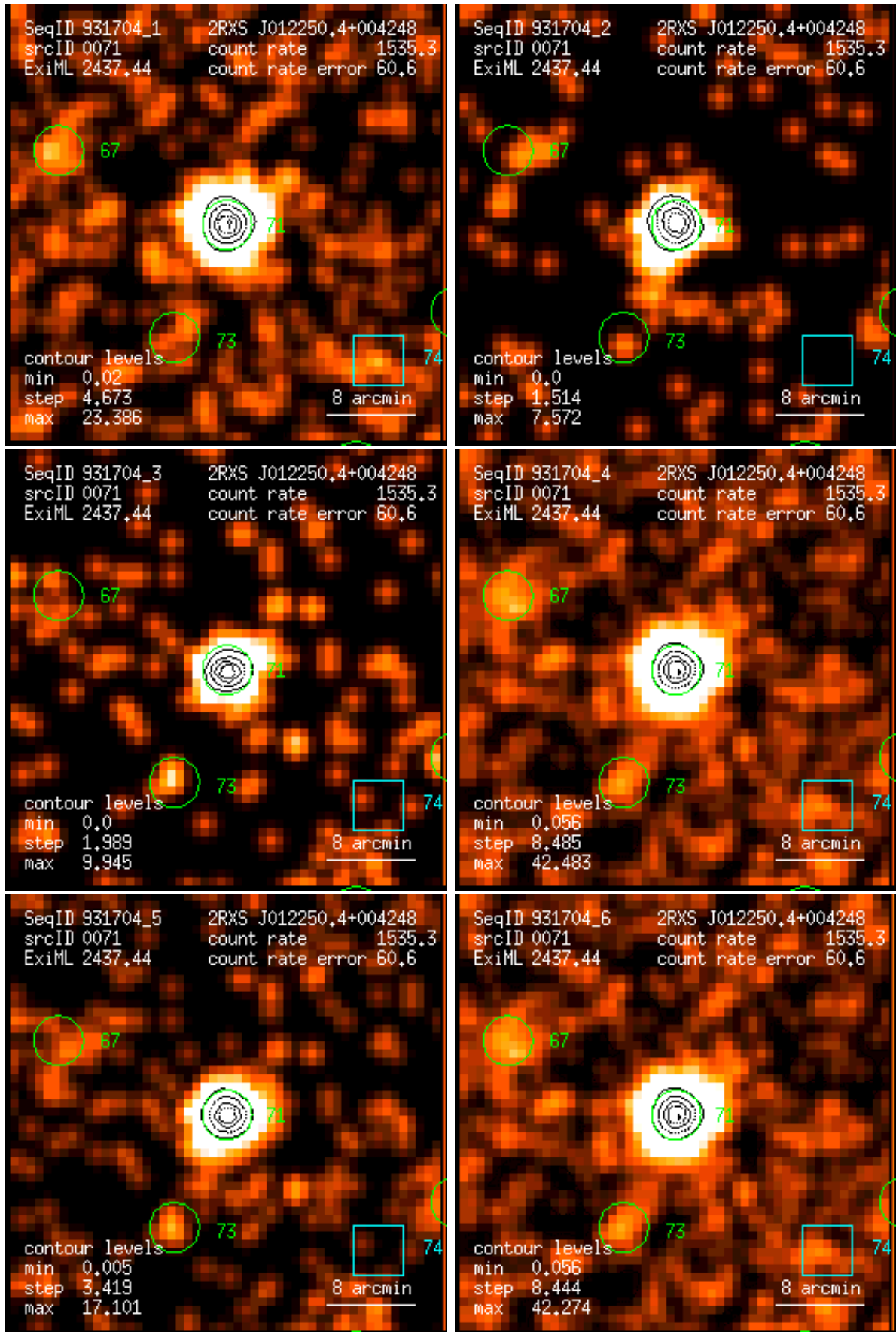
Figure 71: RASS 931704: detection 0071: band rate images, Gaussian filter: (1) PSPC channels 11 – 41, (2) 52 – 90, (3) 91 – 201, (4) 11 – 235, (5) 52 – 201, (6) 11 – 201. Broad band rates in counts/ks. Band rate contour levels in counts/ks/arcmin 2 .
