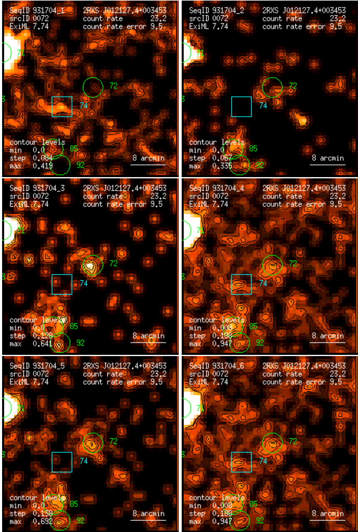
Figure 72: RASS 931704: detection 0072: band rate images, Gaussian filter: (1) PSPC channels 11 – 41, (2) 52 – 90, (3) 91 – 201, (4) 11 – 235, (5) 52 – 201, (6) 11 – 201. Broad band rates in counts/ks. Band rate contour levels in counts/ks/arcmin 2 .
