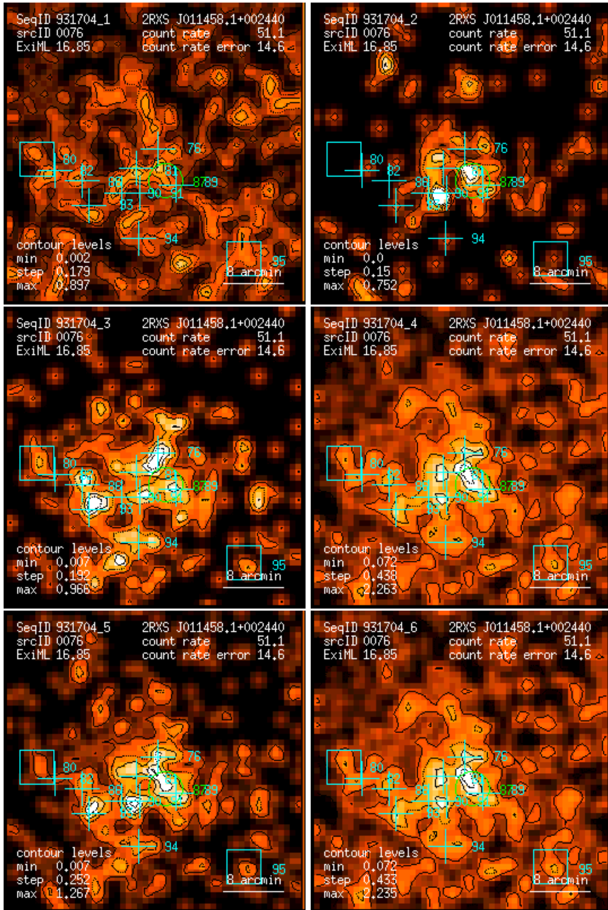
Figure 76: RASS 931704: detection 0076: band rate images, Gaussian filter: (1) PSPC channels 11 – 41, (2) 52 – 90, (3) 91 – 201, (4) 11 – 235, (5) 52 – 201, (6) 11 – 201. Broad band rates in counts/ks. Band rate contour levels in counts/ks/arcmin 2 .
