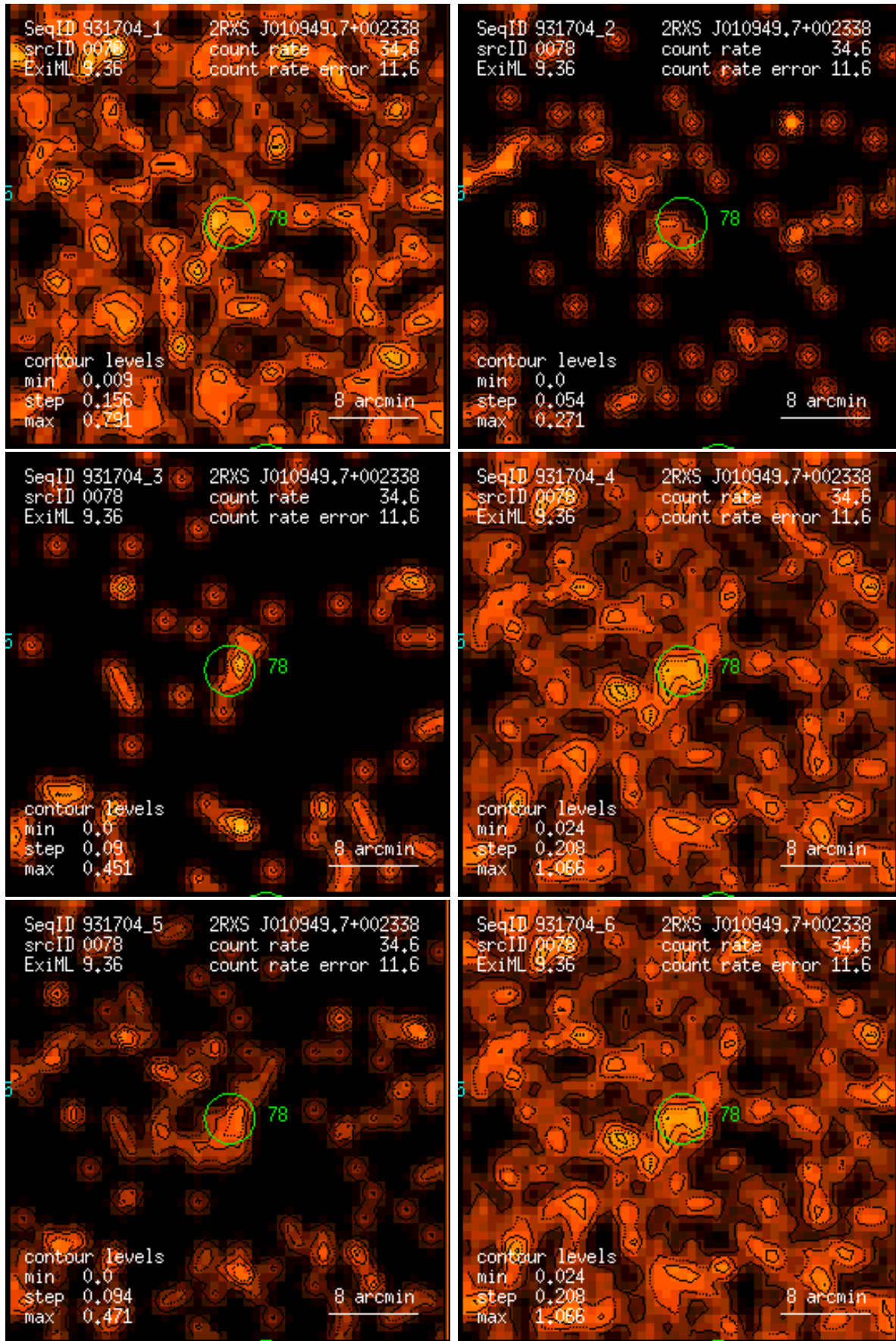
Figure 78: RASS 931704: detection 0078: band rate images, Gaussian filter: (1) PSPC channels 11 – 41, (2) 52 – 90, (3) 91 – 201, (4) 11 – 235, (5) 52 – 201, (6) 11 – 201. Broad band rates in counts/ks. Band rate contour levels in counts/ks/arcmin 2 .
