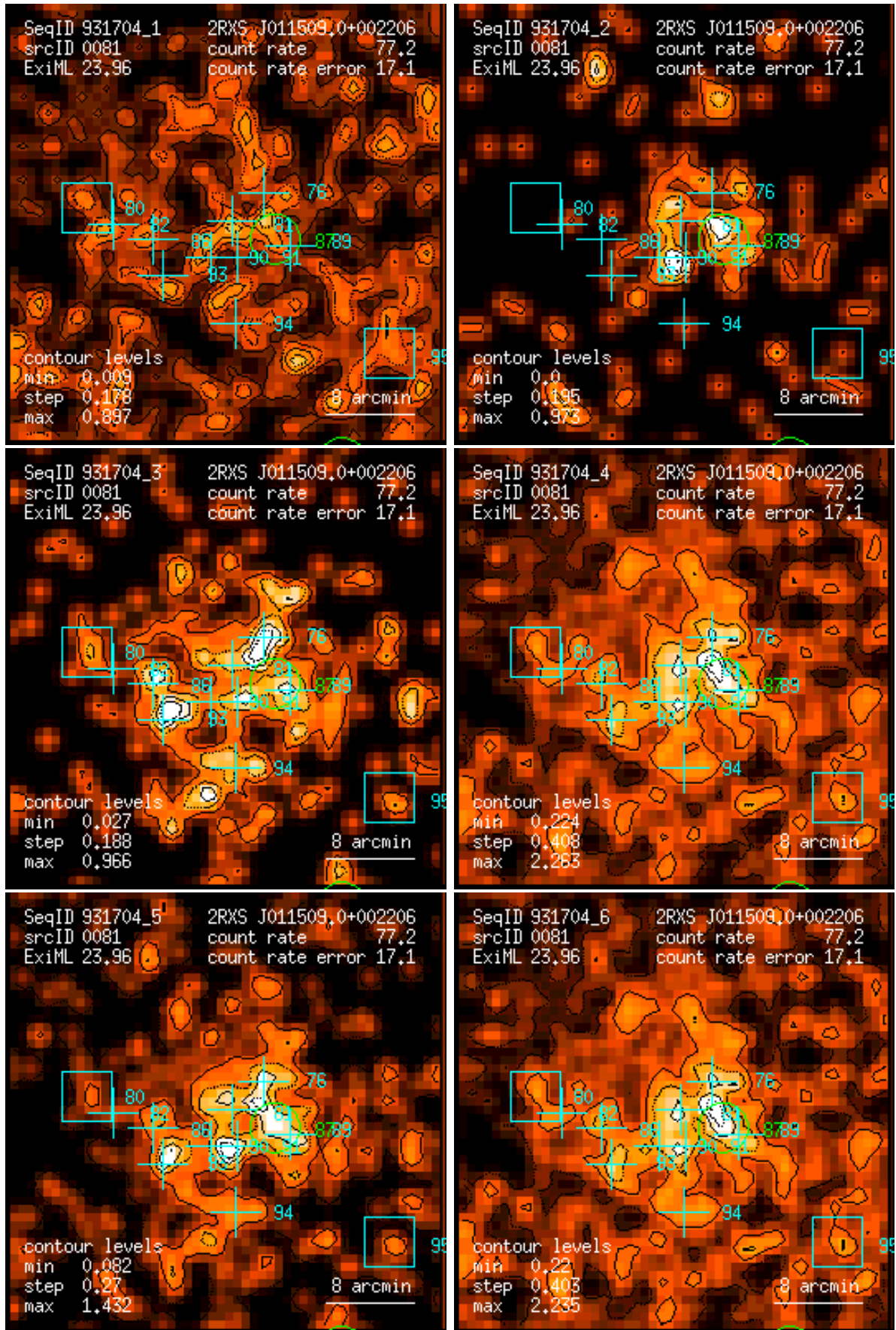
Figure 81: RASS 931704: detection 0081: band rate images, Gaussian filter: (1) PSPC channels 11 – 41, (2) 52 – 90, (3) 91 – 201, (4) 11 – 235, (5) 52 – 201, (6) 11 – 201. Broad band rates in counts/ks. Band rate contour levels in counts/ks/arcmin 2 .
