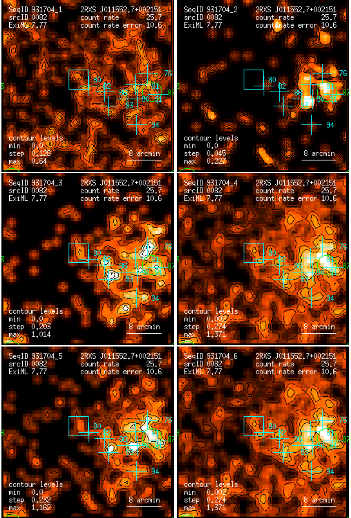
Figure 82: RASS 931704: detection 0082: band rate images, Gaussian filter: (1) PSPC channels 11 – 41, (2) 52 – 90, (3) 91 – 201, (4) 11 – 235, (5) 52 – 201, (6) 11 – 201. Broad band rates in counts/ks. Band rate contour levels in counts/ks/arcmin 2 .
