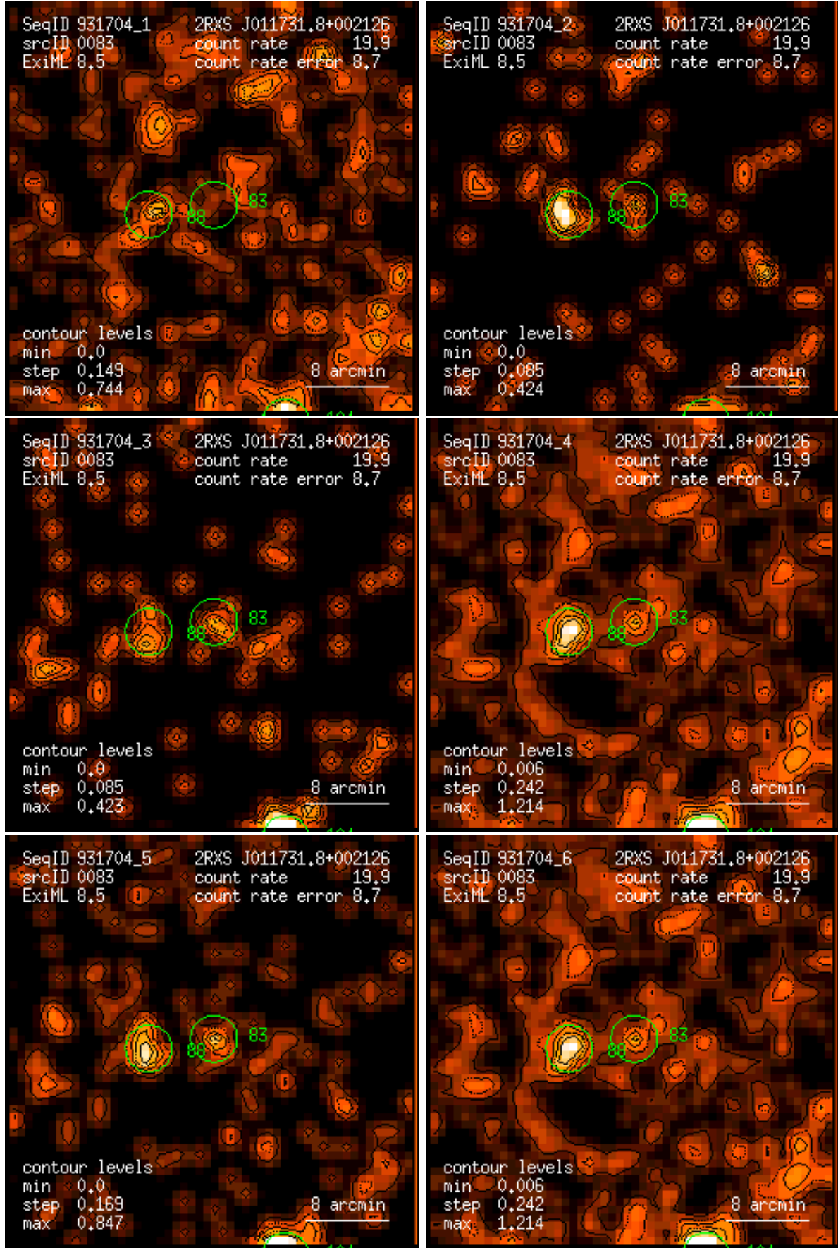
Figure 83: RASS 931704: detection 0083: band rate images, Gaussian filter: (1) PSPC channels 11 – 41, (2) 52 – 90, (3) 91 – 201, (4) 11 – 235, (5) 52 – 201, (6) 11 – 201. Broad band rates in counts/ks. Band rate contour levels in counts/ks/arcmin 2 .
