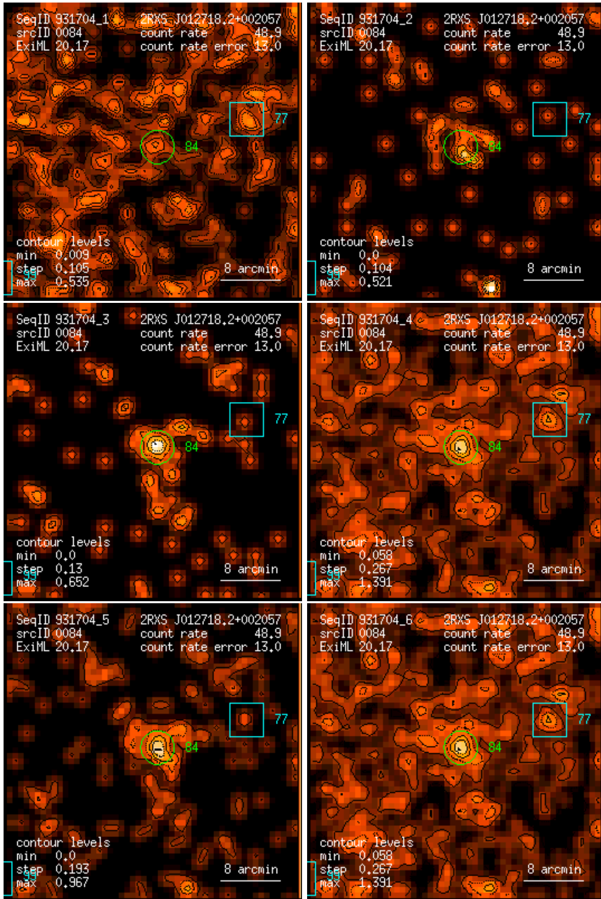
Figure 84: RASS 931704: detection 0084: band rate images, Gaussian filter: (1) PSPC channels 11 – 41, (2) 52 – 90, (3) 91 – 201, (4) 11 – 235, (5) 52 – 201, (6) 11 – 201. Broad band rates in counts/ks. Band rate contour levels in counts/ks/arcmin 2 .
