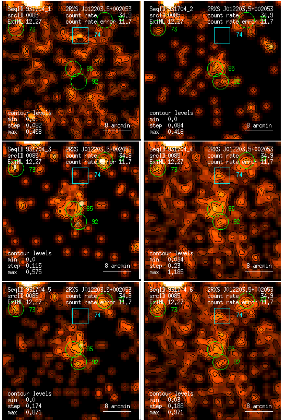
Figure 85: RASS 931704: detection 0085: band rate images, Gaussian filter: (1) PSPC channels 11 – 41, (2) 52 – 90, (3) 91 – 201, (4) 11 – 235, (5) 52 – 201, (6) 11 – 201. Broad band rates in counts/ks. Band rate contour levels in counts/ks/arcmin 2 .
