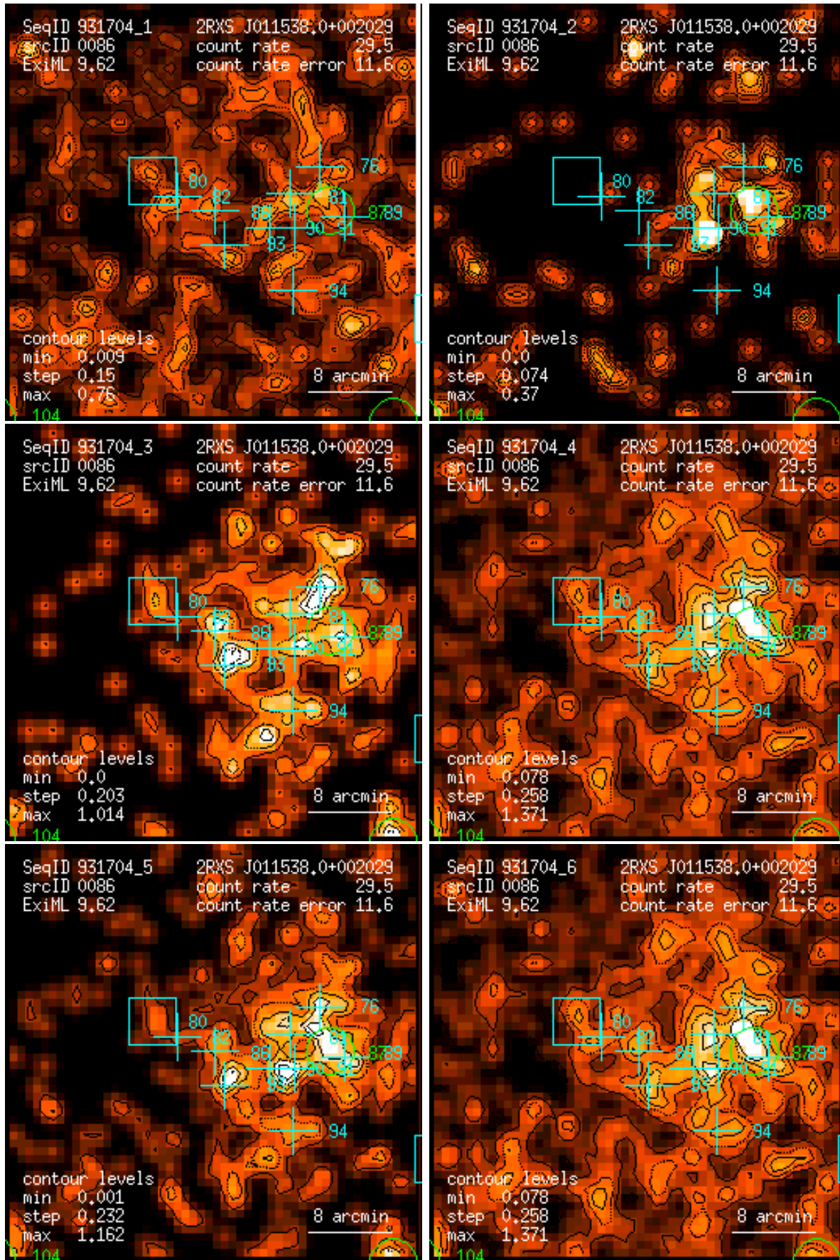
Figure 86: RASS 931704: detection 0086: band rate images, Gaussian filter: (1) PSPC channels 11 – 41, (2) 52 – 90, (3) 91 – 201, (4) 11 – 235, (5) 52 – 201, (6) 11 – 201. Broad band rates in counts/ks. Band rate contour levels in counts/ks/arcmin 2 .
