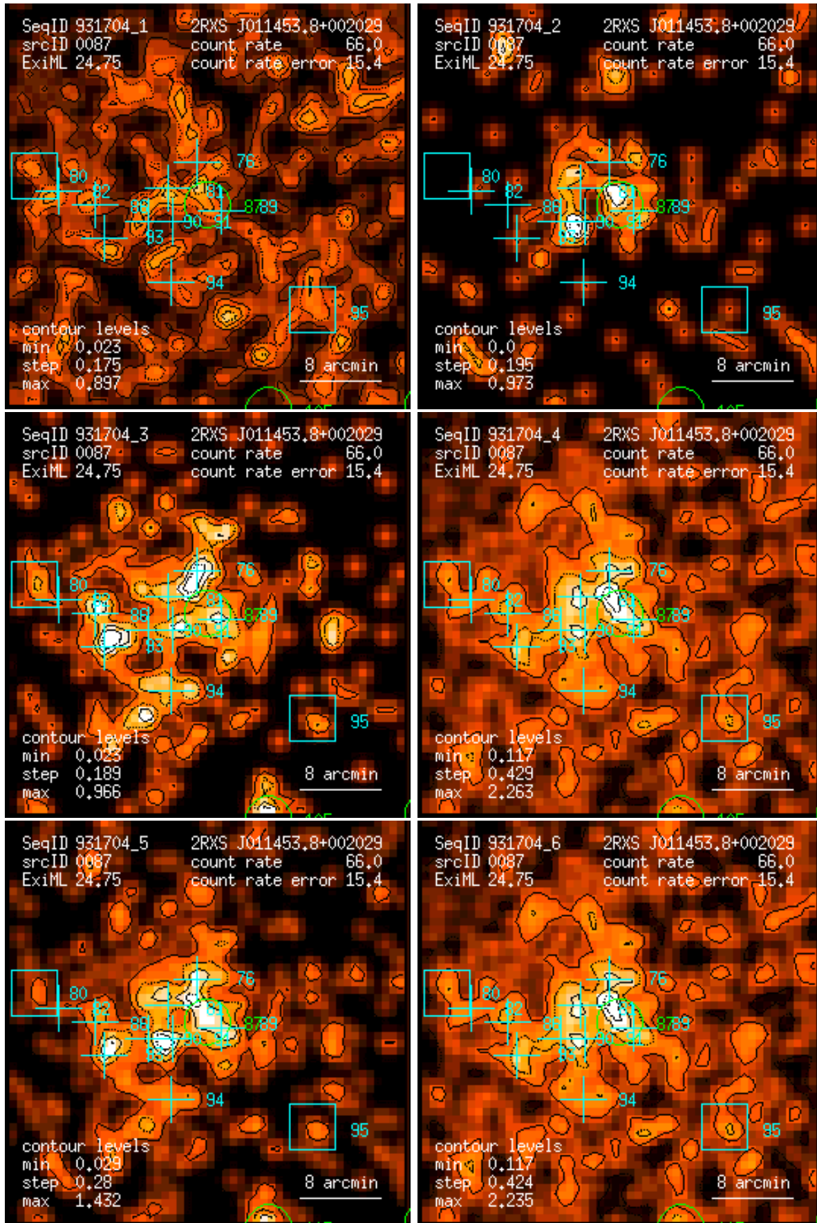
Figure 87: RASS 931704: detection 0087: band rate images, Gaussian filter: (1) PSPC channels 11 – 41, (2) 52 – 90, (3) 91 – 201, (4) 11 – 235, (5) 52 – 201, (6) 11 – 201. Broad band rates in counts/ks. Band rate contour levels in counts/ks/arcmin 2 .
