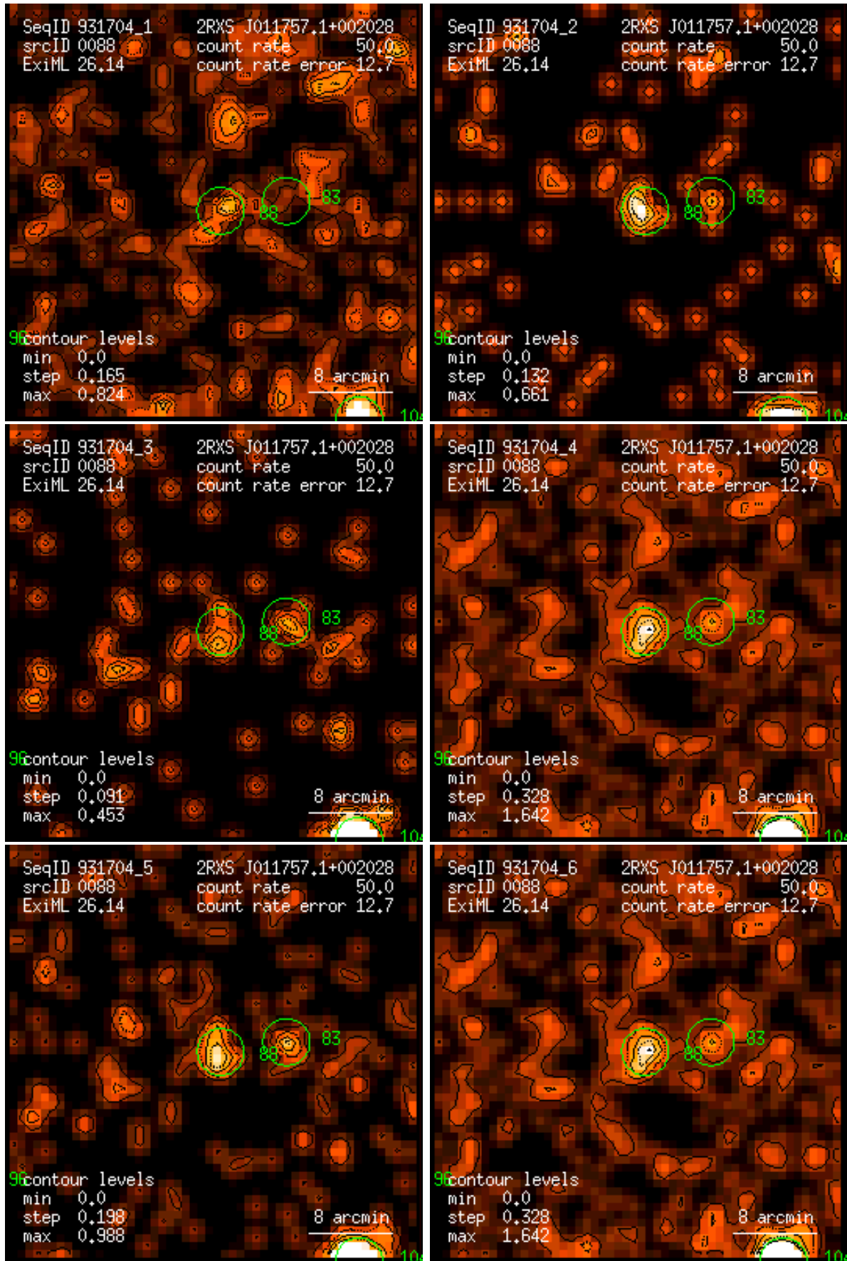
Figure 88: RASS 931704: detection 0088: band rate images, Gaussian filter: (1) PSPC channels 11 – 41, (2) 52 – 90, (3) 91 – 201, (4) 11 – 235, (5) 52 – 201, (6) 11 – 201. Broad band rates in counts/ks. Band rate contour levels in counts/ks/arcmin 2 .
