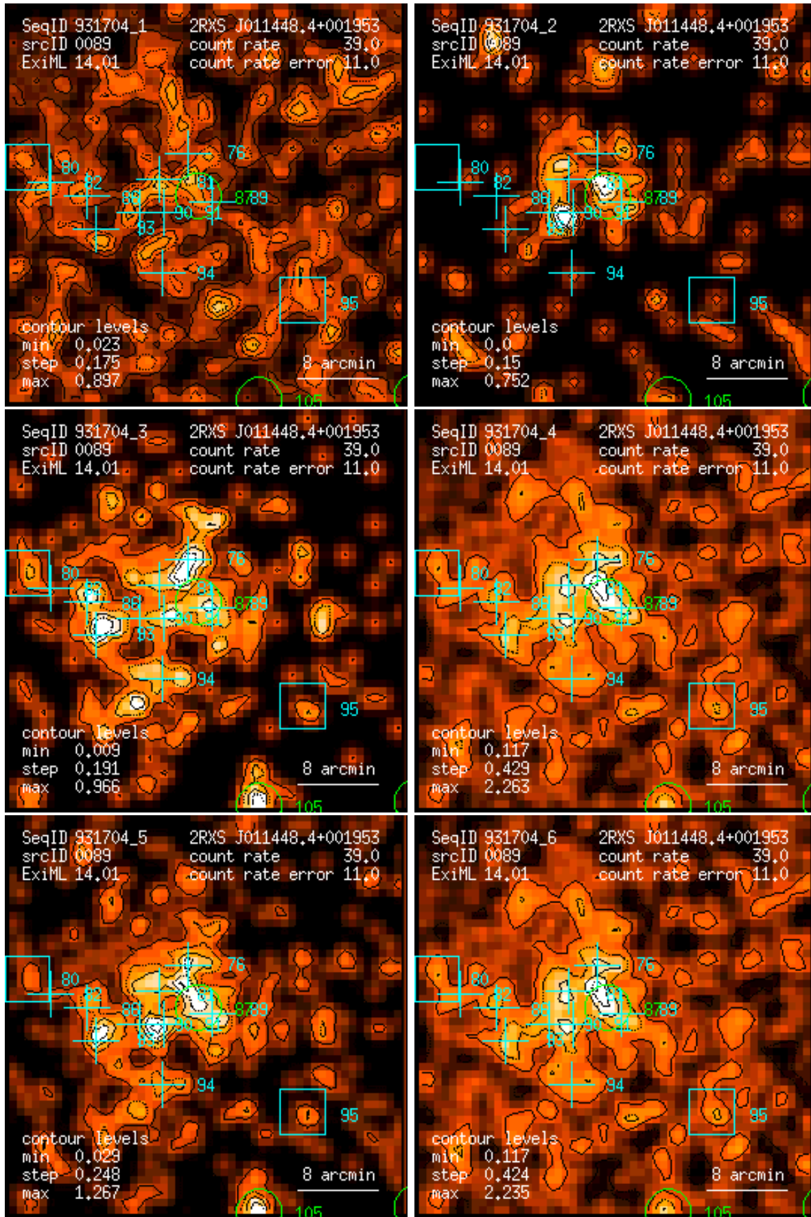
Figure 89: RASS 931704: detection 0089: band rate images, Gaussian filter: (1) PSPC channels 11 – 41, (2) 52 – 90, (3) 91 – 201, (4) 11 – 235, (5) 52 – 201, (6) 11 – 201. Broad band rates in counts/ks. Band rate contour levels in counts/ks/arcmin 2 .
