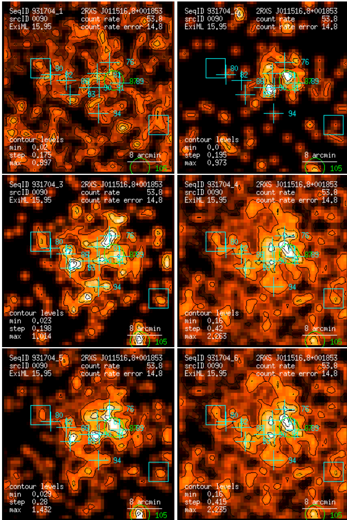
Figure 90: RASS 931704: detection 0090: band rate images, Gaussian filter: (1) PSPC channels 11 – 41, (2) 52 – 90, (3) 91 – 201, (4) 11 – 235, (5) 52 – 201, (6) 11 – 201. Broad band rates in counts/ks. Band rate contour levels in counts/ks/arcmin 2 .
