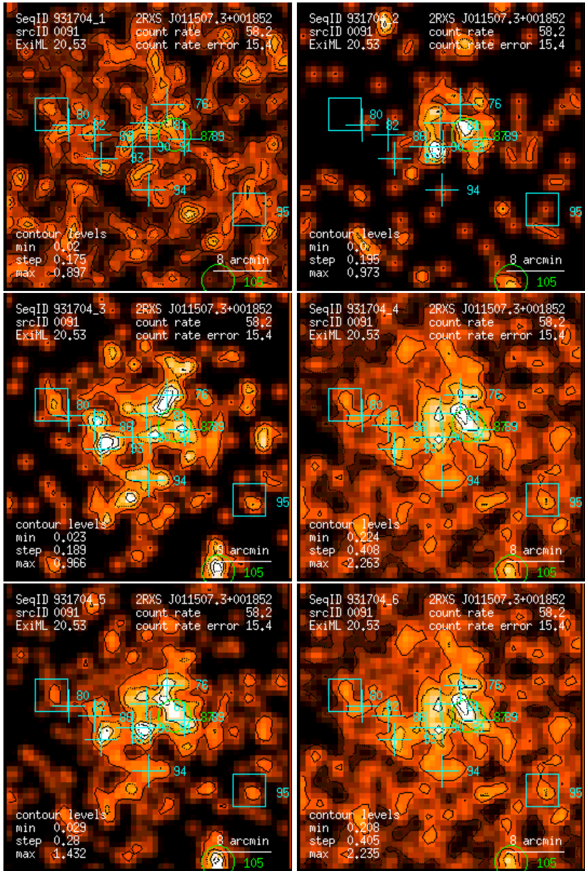
Figure 91: RASS 931704: detection 0091: band rate images, Gaussian filter: (1) PSPC channels 11 – 41, (2) 52 – 90, (3) 91 – 201, (4) 11 – 235, (5) 52 – 201, (6) 11 – 201. Broad band rates in counts/ks. Band rate contour levels in counts/ks/arcmin 2 .
