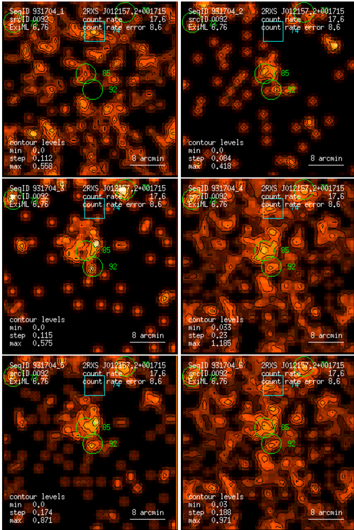
Figure 92: RASS 931704: detection 0092: band rate images, Gaussian filter: (1) PSPC channels 11 – 41, (2) 52 – 90, (3) 91 – 201, (4) 11 – 235, (5) 52 – 201, (6) 11 – 201. Broad band rates in counts/ks. Band rate contour levels in counts/ks/arcmin 2 .
