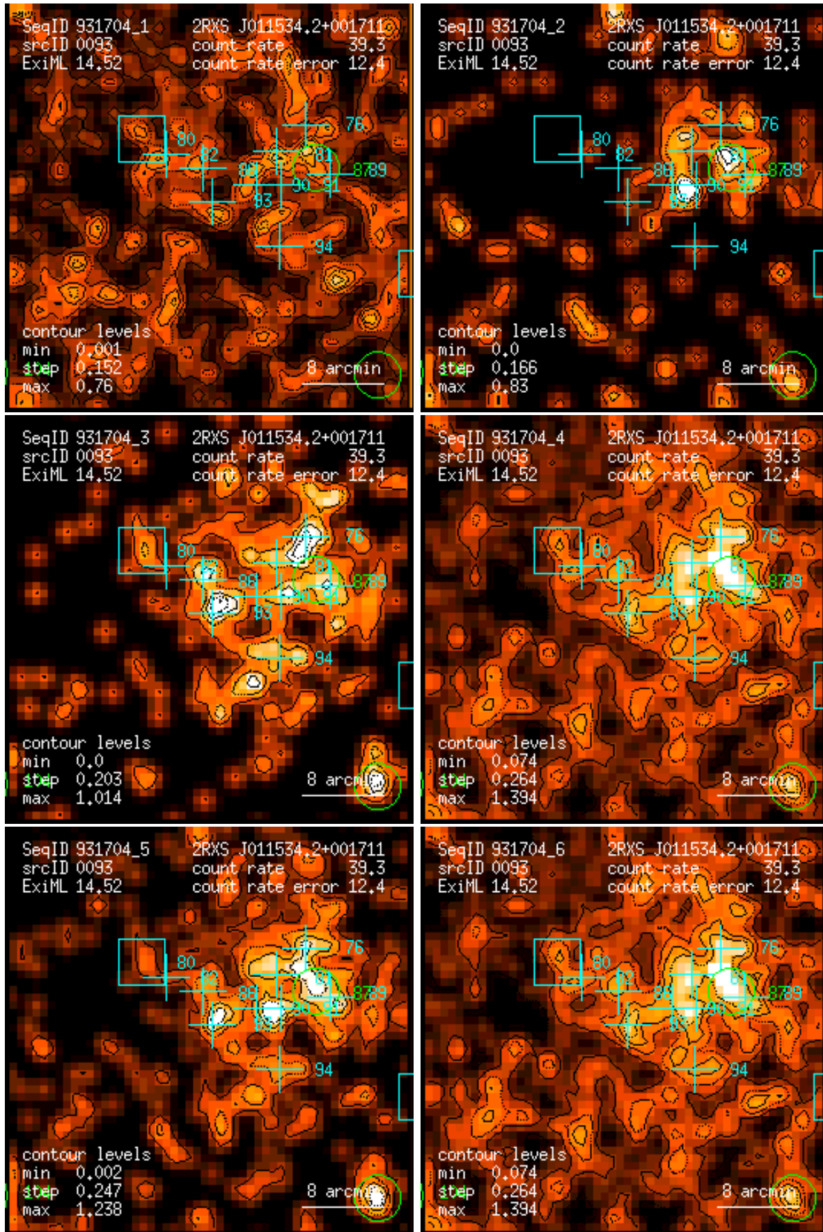
Figure 93: RASS 931704: detection 0093: band rate images, Gaussian filter: (1) PSPC channels 11 – 41, (2) 52 – 90, (3) 91 – 201, (4) 11 – 235, (5) 52 – 201, (6) 11 – 201. Broad band rates in counts/ks. Band rate contour levels in counts/ks/arcmin 2 .
