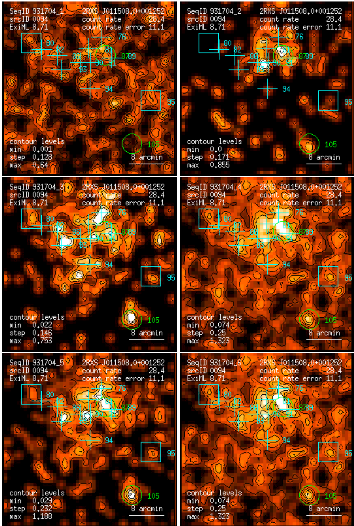
Figure 94: RASS 931704: detection 0094: band rate images, Gaussian filter: (1) PSPC channels 11 – 41, (2) 52 – 90, (3) 91 – 201, (4) 11 – 235, (5) 52 – 201, (6) 11 – 201. Broad band rates in counts/ks. Band rate contour levels in counts/ks/arcmin 2 .
