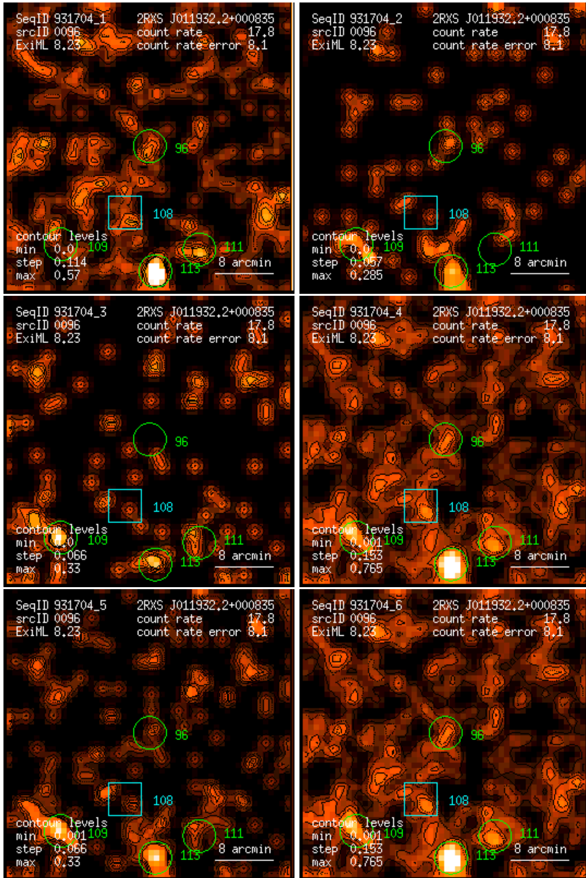
Figure 96: RASS 931704: detection 0096: band rate images, Gaussian filter: (1) PSPC channels 11 – 41, (2) 52 – 90, (3) 91 – 201, (4) 11 – 235, (5) 52 – 201, (6) 11 – 201. Broad band rates in counts/ks. Band rate contour levels in counts/ks/arcmin 2 .
